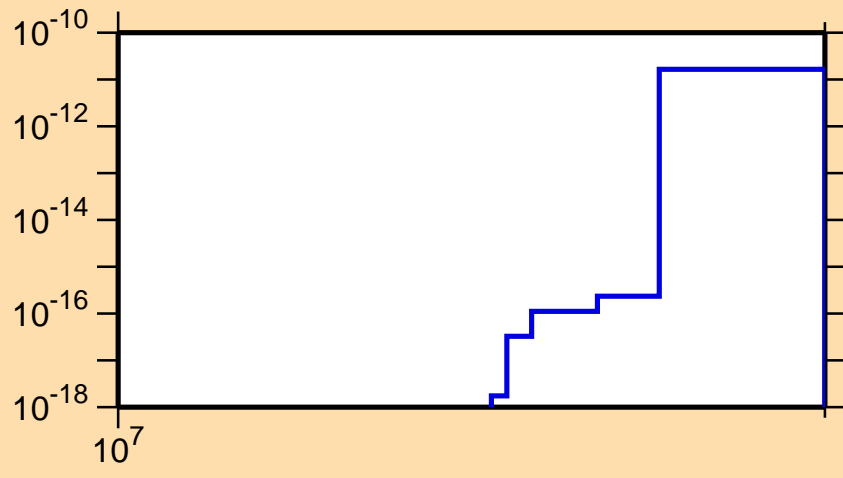
\sigma vs. E for ^{56}\text{Co} (mt 45)
