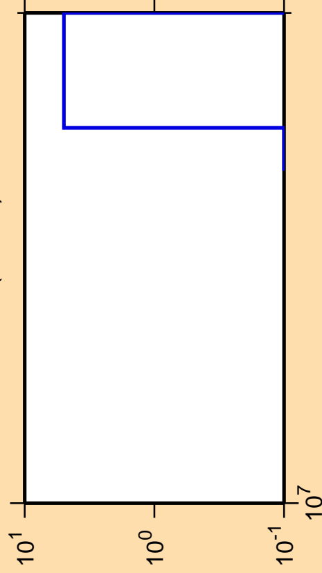
\Delta\sigma/\sigma vs. E for ^{56}\text{Co} (mt 34)
