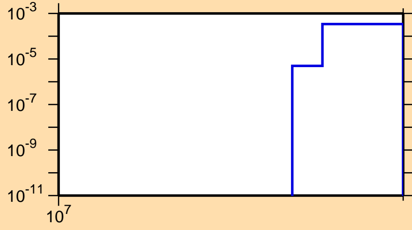
\sigma vs. E for ^{56}\text{Co}(n,2np)
