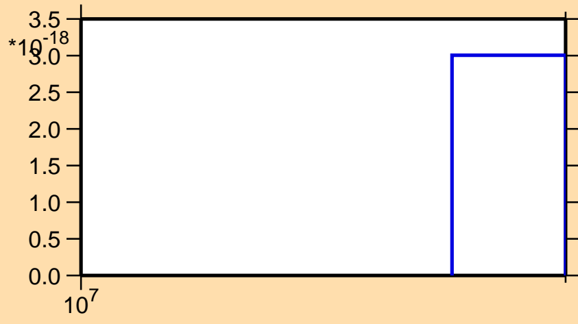
\sigma vs. E for ^{56}\text{Co}(n,2n\alpha)
