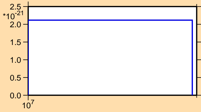
\sigma vs. E for ^{57}\text{Co} (mt 34)
