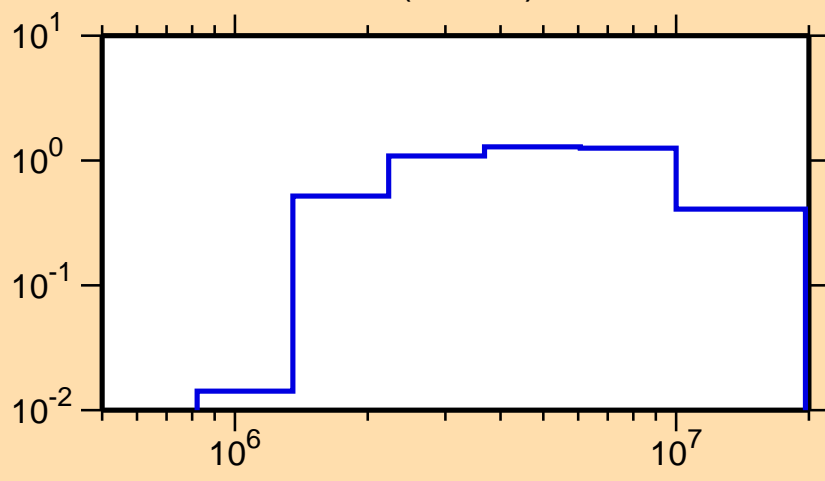
\sigma vs. E for ^{57}\text{Co}(n,\text{inel.})
