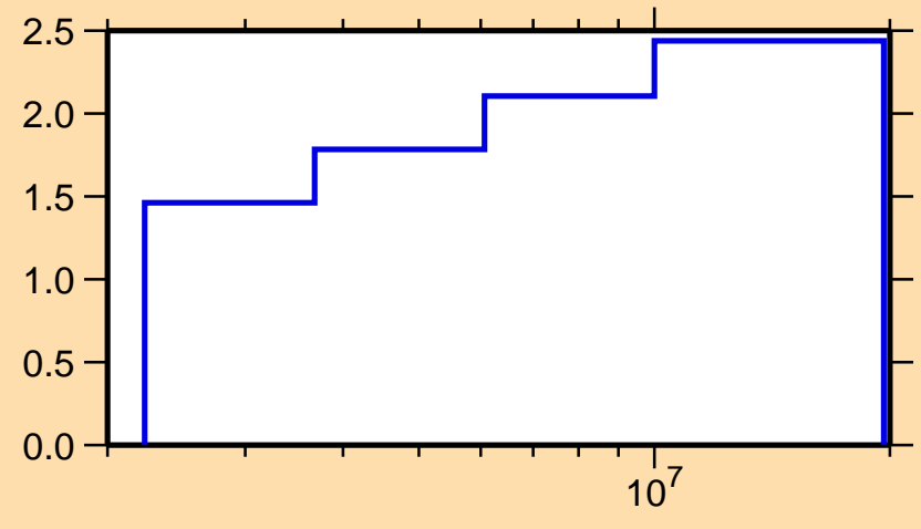
\Delta\sigma/\sigma vs. E for ^{57}\text{Co}(n,n\text{nonel.})
