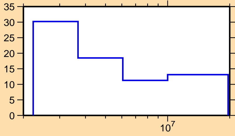
\Delta\sigma/\sigma vs. E for ^{57}\text{Co}(n,n\text{cont.})
