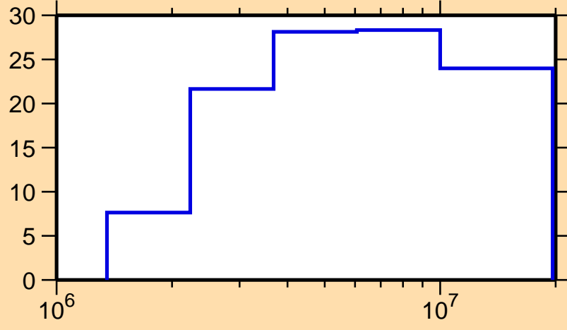
\Delta\sigma/\sigma vs. E for ^{58}\text{Co}(n,n_1)
