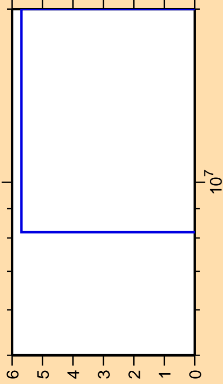
\Delta\sigma/\sigma vs. E for ^{58}\text{Co}(n,2n\alpha)
