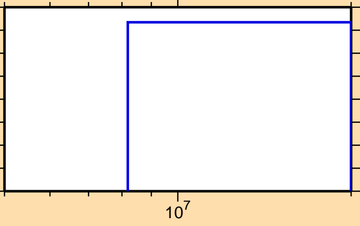
\sigma vs. E for ^{60}\text{Co}(n,\text{pt})
