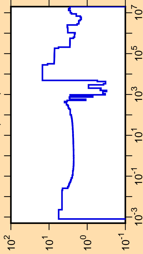
\Delta\sigma/\sigma vs. E for ^{62}\text{Co}(n,\text{tot.})
