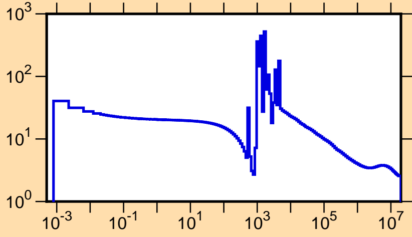
\sigma vs. E for ^{62}\text{Co}(n,\text{tot.})
