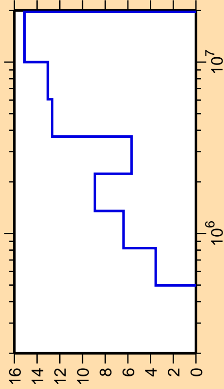
\Delta\sigma/\sigma vs. E for ^{62}\text{Co}(n,n_4)
