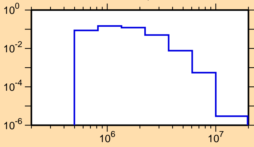
\sigma vs. E for ^{62}\text{Co}(n,n_4)
