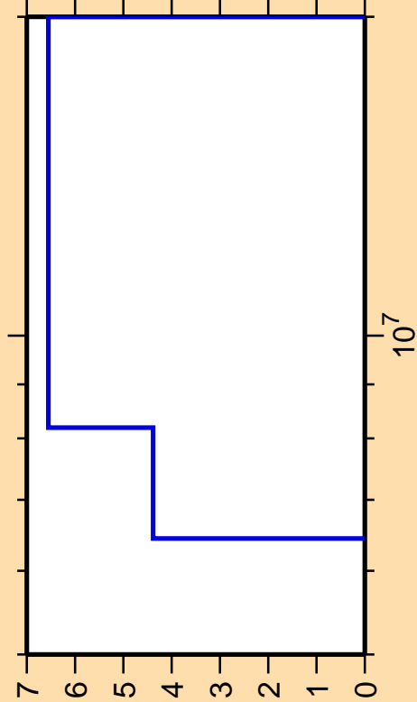
\Delta\sigma/\sigma vs. E for ^{62}\text{Co}(n,n\text{cont.})
