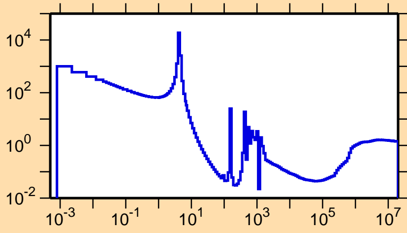
\sigma vs. E for ^{62}\text{Co}(n,\text{nonel.})
