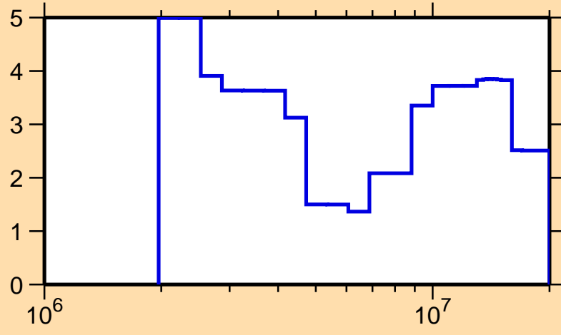
\Delta\sigma/\sigma vs. E for ^{62}\text{Co}(n,\text{el.})
