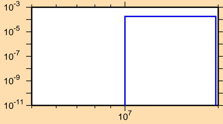
\sigma vs. E for ^{62}\text{Co}(n,n\alpha)
