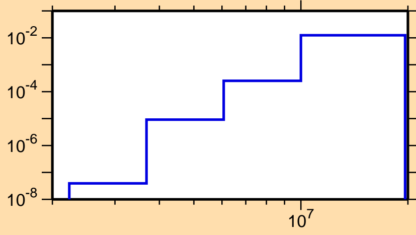
\sigma vs. E for ^{62}\text{Co}(n,p)
