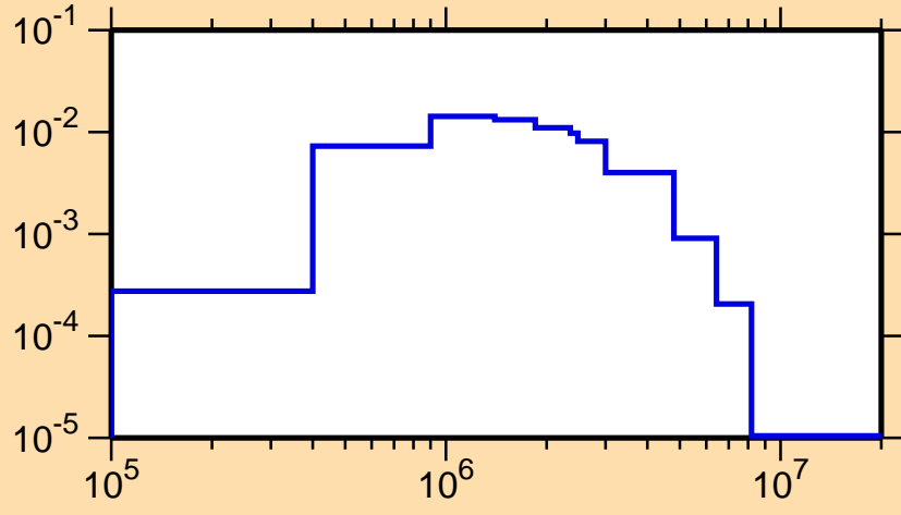
\sigma vs. E for ^{62}\text{Co}(n,n_2)
