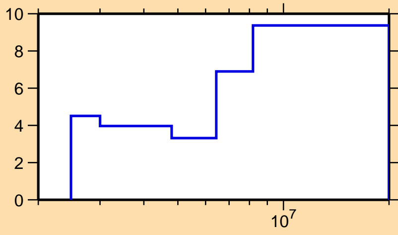
\Delta\sigma/\sigma vs. E for ^{62}\text{Co}(n,n\text{cont.})
