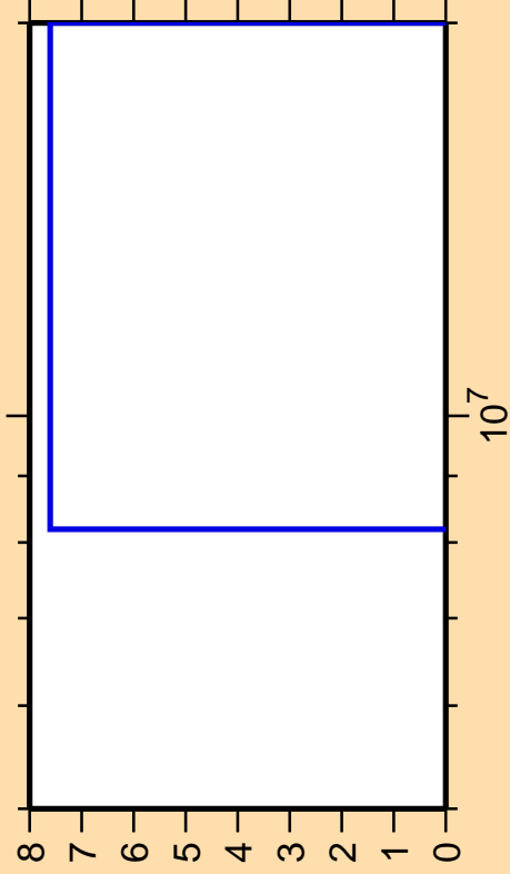
\Delta\sigma/\sigma vs. E for ^{62}\text{Co}(n,np)
