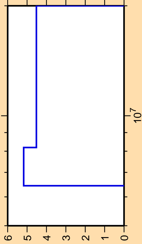
\Delta\sigma/\sigma vs. E for ^{62}\text{Co}(n,2n)
