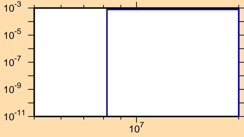
\sigma vs. E for ^{62}\text{Co}(n,d)
