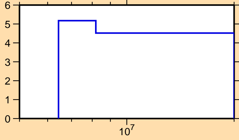
\Delta\sigma/\sigma vs. E for ^{62}\text{Co}(n,2n)
