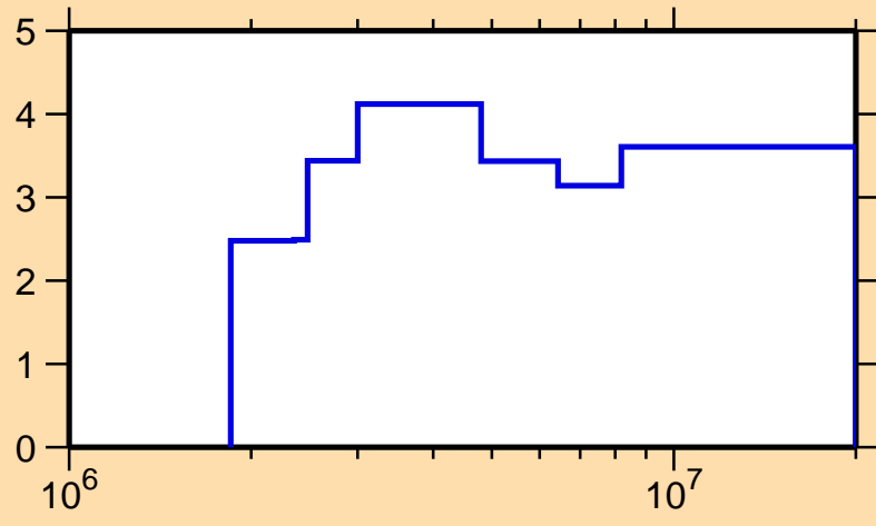
\Delta\sigma/\sigma vs. E for ^{62}\text{Co}(n,n\text{nonel.})
