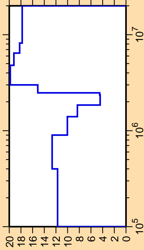
\Delta\sigma/\sigma vs. E for ^{62}\text{Co}(n,n_2)
