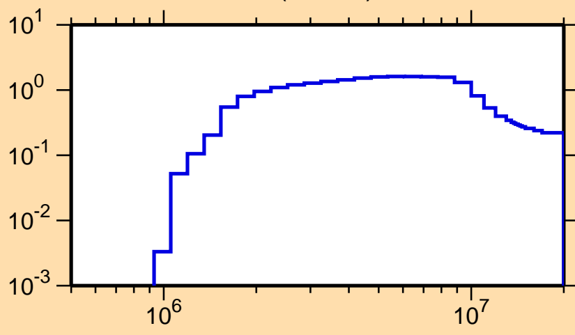
\sigma vs. E for ^{63}\text{Co}(n,\text{inel.})
