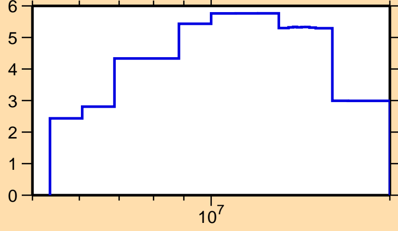
\Delta\sigma/\sigma vs. E for ^{63}\text{Co}(n,\text{el.})
