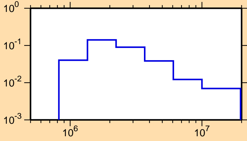
\sigma vs. E for ^{63}\text{Co}(n,n_1)
