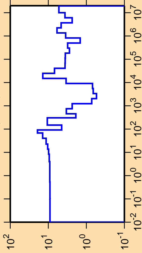
\Delta\sigma/\sigma vs. E for ^{63}\text{Co}(n,\text{el.})
