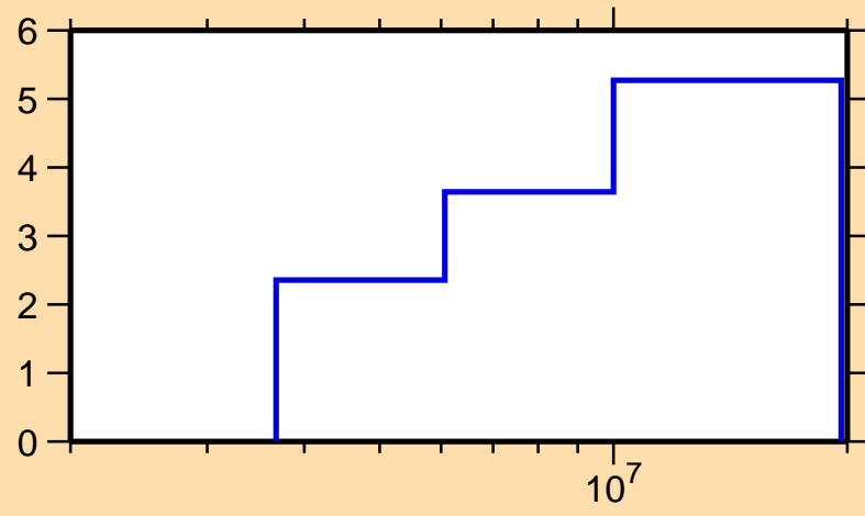
\Delta\sigma/\sigma vs. E for ^{63}\text{Co}(n,\text{el.})
