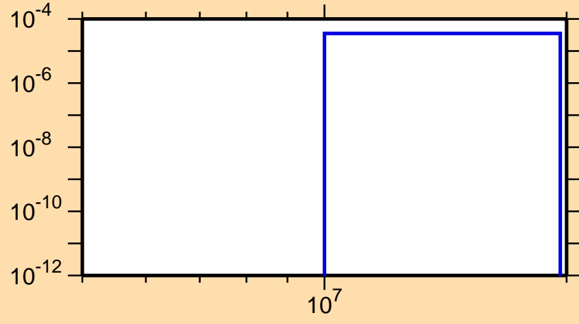
\sigma vs. E for ^{63}\text{Co}(n,n\alpha)
