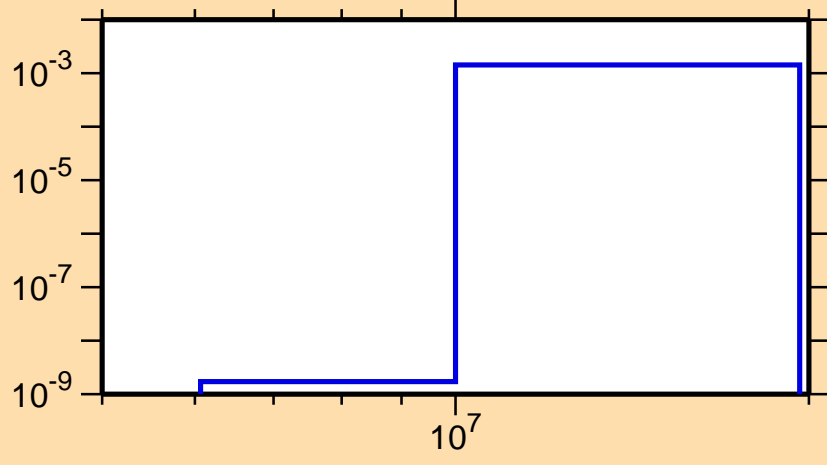
\sigma vs. E for ^{63}\text{Co}(n,d)
