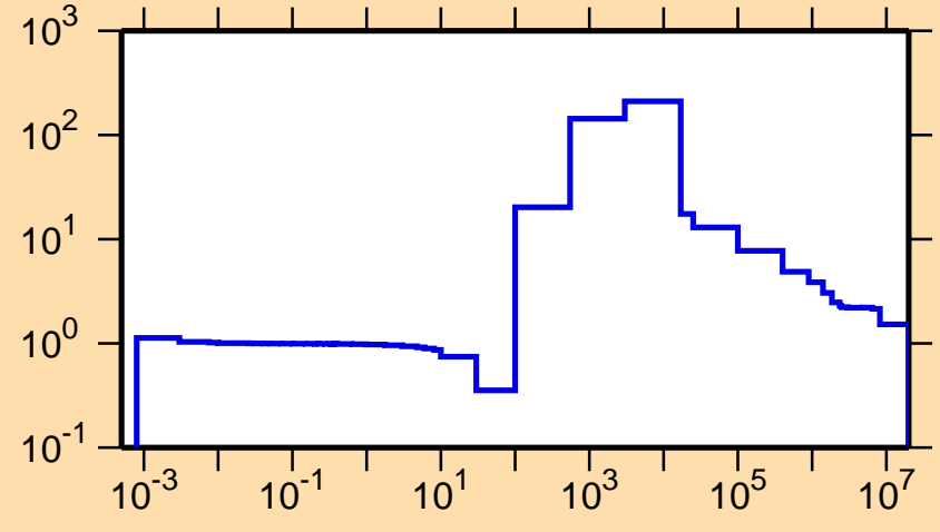
\sigma vs. E for ^{63}\text{Co}(n,\text{el.})
