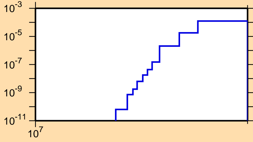
\sigma vs. E for ^{65}\text{Co}(n,n\alpha)
