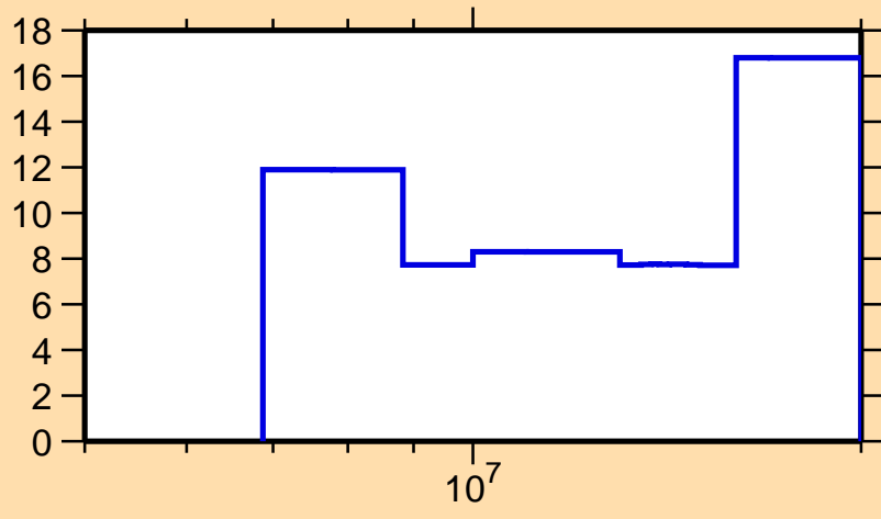
\Delta\sigma/\sigma vs. E for ^{65}\text{Co}(n,2n)
