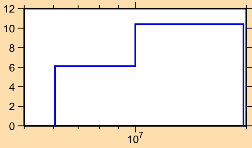
\Delta\sigma/\sigma vs. E for ^{65}\text{Co}(n,el.)
