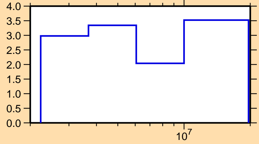
\Delta\sigma/\sigma vs. E for ^{65}\text{Co}(n,n\text{nonel.})
