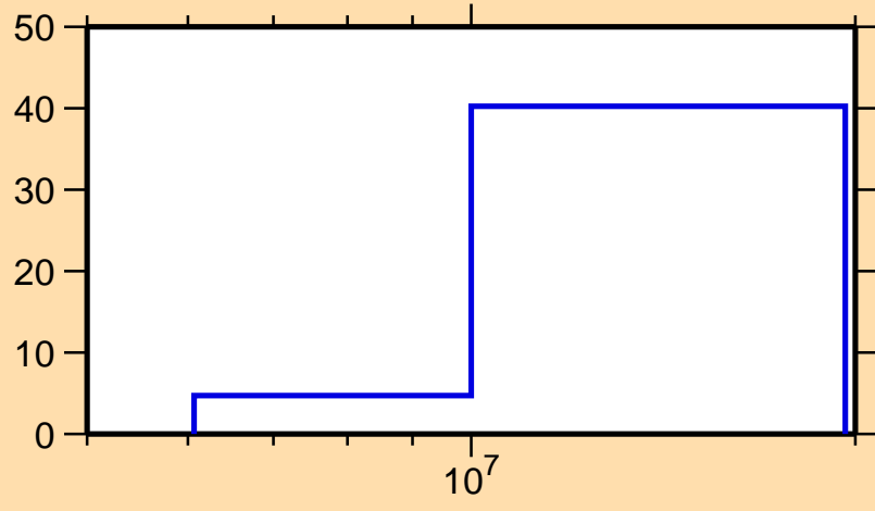
\Delta\sigma/\sigma vs. E for ^{65}\text{Co}(n,n\text{cont.})
