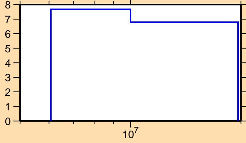
\Delta\sigma/\sigma vs. E for ^{65}\text{Co}(n,2n)
