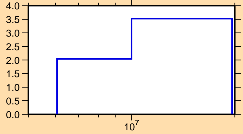
\Delta\sigma/\sigma vs. E for ^{65}\text{Co}(n,\text{nonel.})
