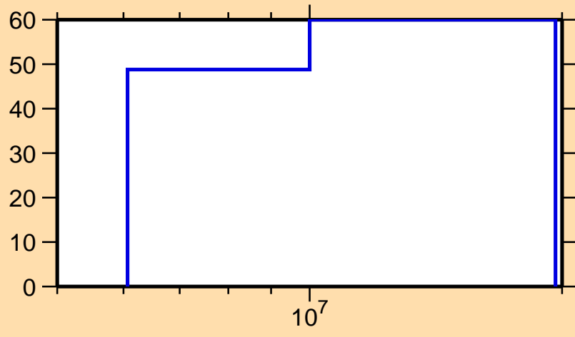
\Delta\sigma/\sigma vs. E for ^{65}\text{Co}(n,\gamma)
