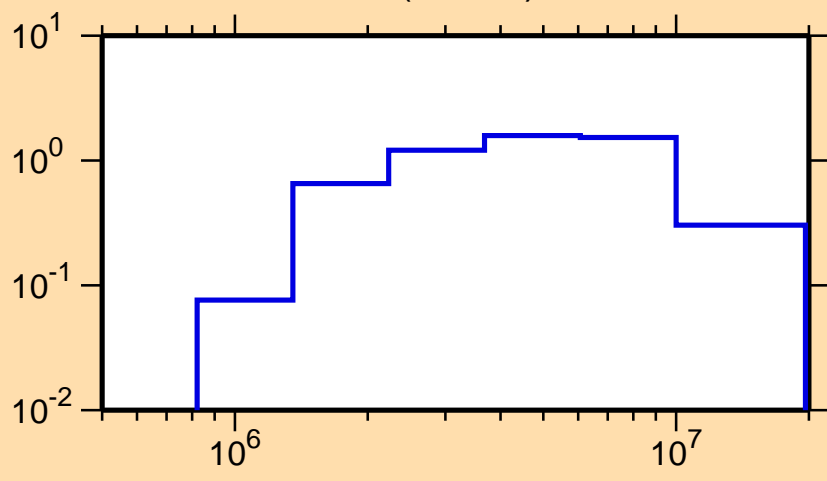
\sigma vs. E for ^{65}\text{Co}(n,\text{inel.})
