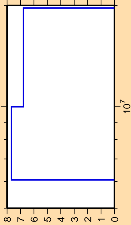
\Delta\sigma/\sigma vs. E for ^{65}\text{Co}(n,2n)
