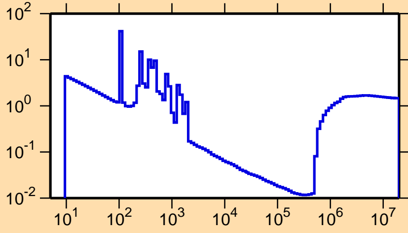
\sigma vs. E for ^{68}\text{Co}(n,\text{nonel.})
