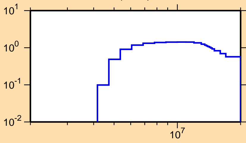
\sigma vs. E for ^{68}\text{Co}(n,2n)
