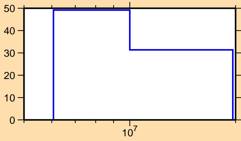
\Delta\sigma/\sigma vs. E for ^{68}\text{Co}(n,p)
