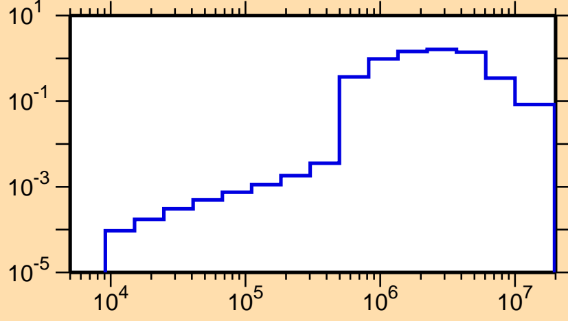
\sigma vs. E for ^{68}\text{Co}(n,\text{inel.})
