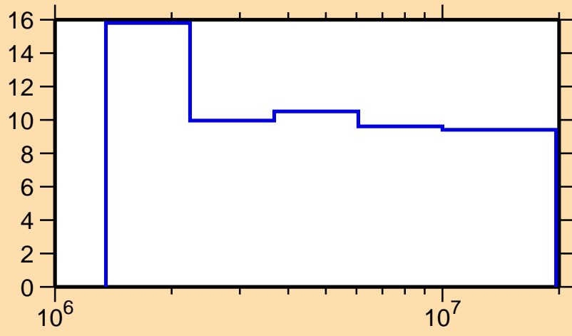
\Delta\sigma/\sigma vs. E for ^{68}\text{Co}(n,n\text{onel.})
