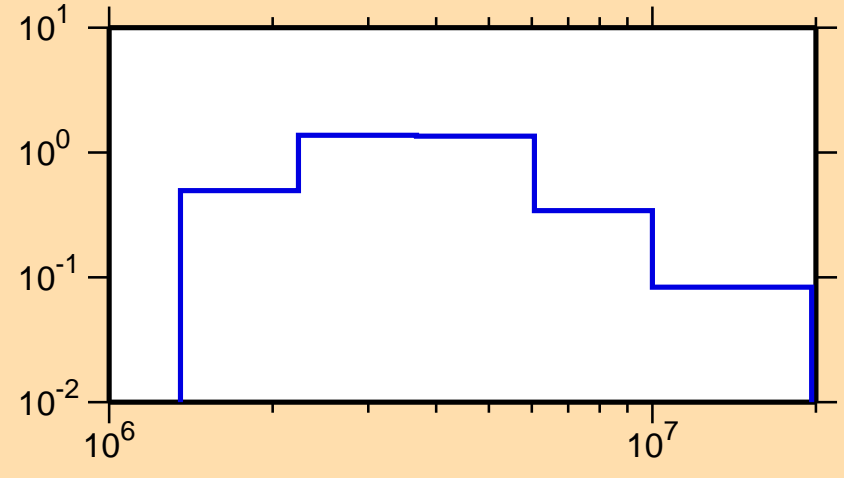
\sigma vs. E for ^{68}\text{Co}(n,n\text{cont.})
