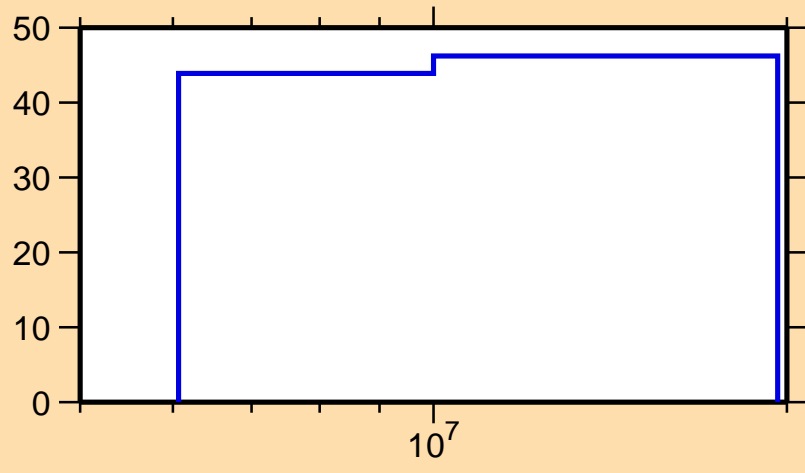
\Delta\sigma/\sigma vs. E for ^{68}\text{Co}(n,ncont.)
