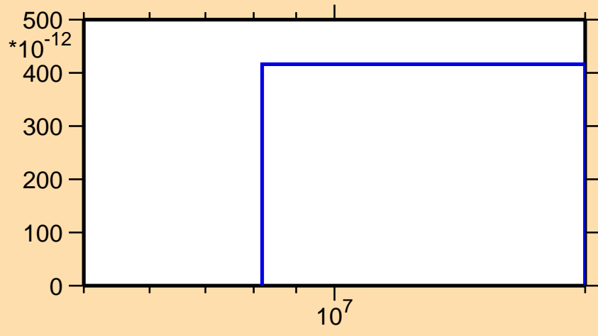
\sigma vs. E for ^{68}\text{Co}(n,2np)
