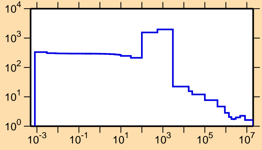
\sigma vs. E for ^{68}\text{Co}(n,\text{el.})
