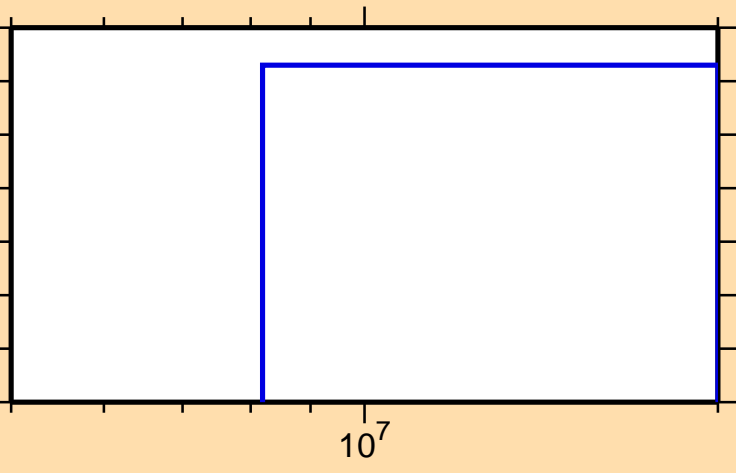
\sigma vs. E for ^{68}\text{Co}(n,d)
