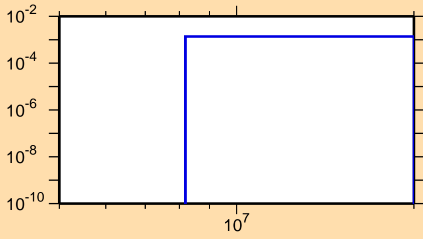
\sigma vs. E for ^{68}\text{Co}(n,p)
