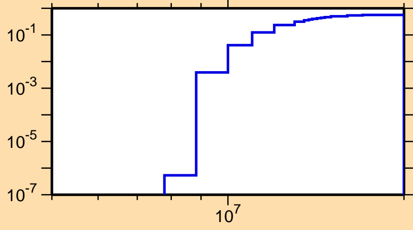
\sigma vs. E for ^{48}\text{Cr}(n,np)
