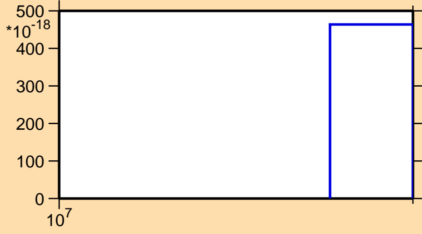
\sigma vs. E for ^{48}\text{Cr}(n,\text{pt})
