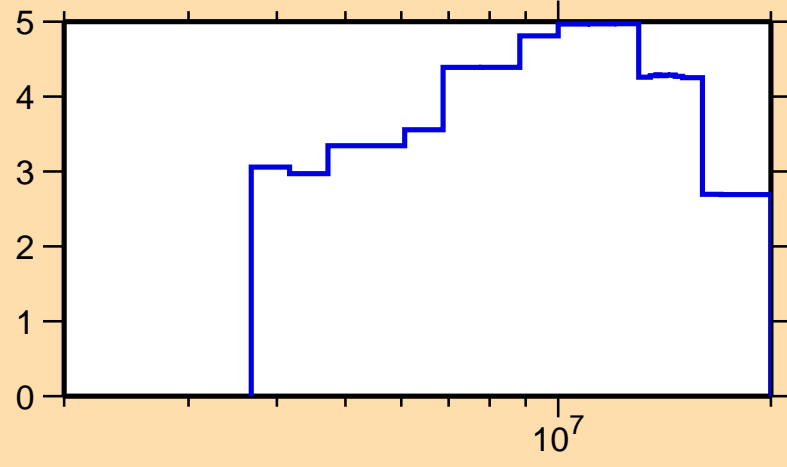
\Delta\sigma/\sigma vs. E for ^{48}\text{Cr}(n,el.)
