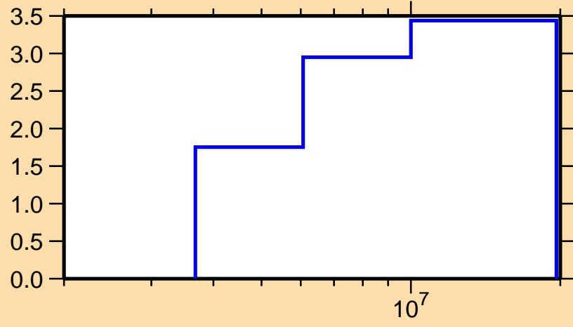
\Delta\sigma/\sigma vs. E for ^{48}\text{Cr}(n,tot.)
