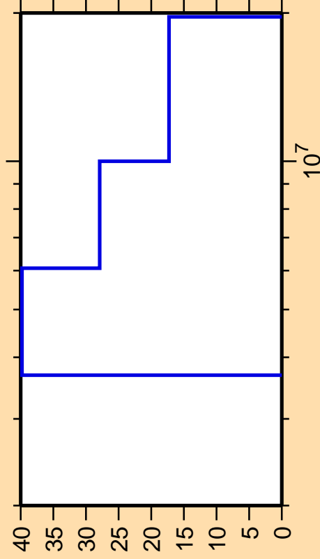
\Delta\sigma/\sigma vs. E for ^{48}\text{Cr}(n,ncont.)
