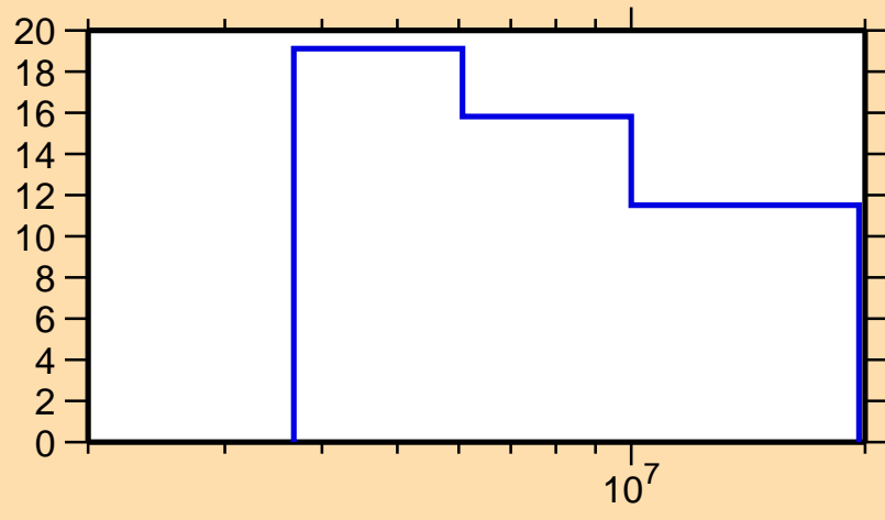
\Delta\sigma/\sigma vs. E for ^{48}\text{Cr}(n,inel.)
