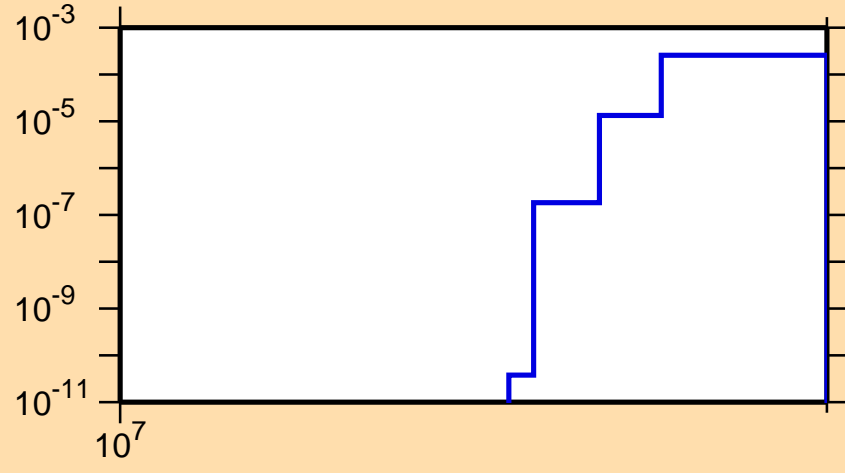
\sigma vs. E for ^{49}\text{Cr}(n,\text{pd})
