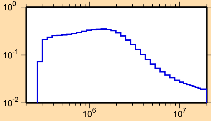
\sigma vs. E for ^{49}\text{Cr}(n,n_1)
