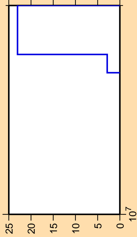
\Delta\sigma/\sigma vs. E for ^{49}\text{Cr}(n,nd)
