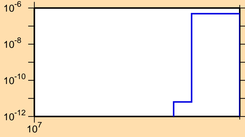
\sigma vs. E for ^{49}\text{Cr}(n,nd)
