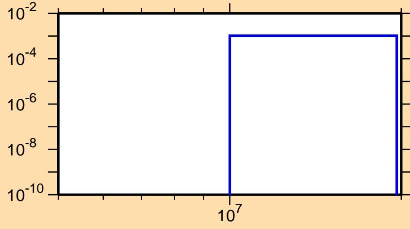
\sigma vs. E for ^{49}\text{Cr}(n,\alpha)
