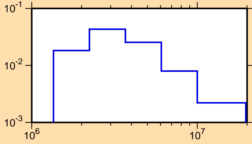
\sigma vs. E for ^{49}\text{Cr}(n,n_3)
