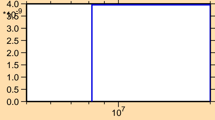
\sigma vs. E for ^{49}\text{Cr}(n,\text{nd})
