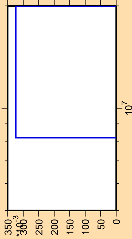
\Delta\sigma/\sigma vs. E for ^{49}\text{Cr}(\text{mt } 34)
