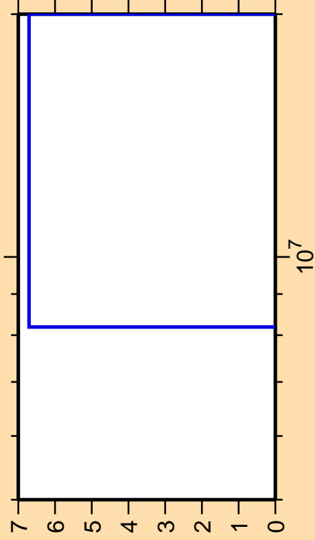
\Delta\sigma/\sigma vs. E for ^{49}\text{Cr}(n,n\text{cont.})
