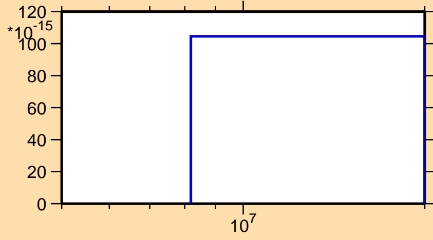
\sigma vs. E for ^{49}\text{Cr}(\text{mt } 34)
