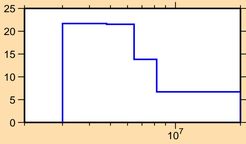
\Delta\sigma/\sigma vs. E for ^{49}\text{Cr}(n,ncont.)
