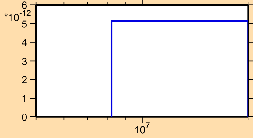
\sigma vs. E for ^{49}\text{Cr}(n,2np)
