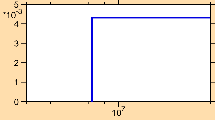
\sigma vs. E for ^{49}\text{Cr}(n,p\alpha)
