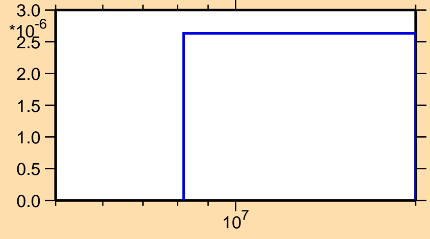
\sigma vs. E for ^{49}\text{Cr}(n,pd)
