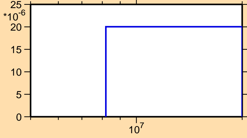
\sigma vs. E for ^{49}\text{Cr}(n,t)
