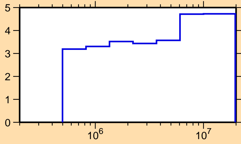
\Delta\sigma/\sigma vs. E for ^{50}\text{Cr}(n,el.)
