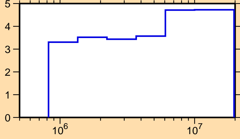
\Delta\sigma/\sigma vs. E for ^{50}\text{Cr}(n,\text{el.})
