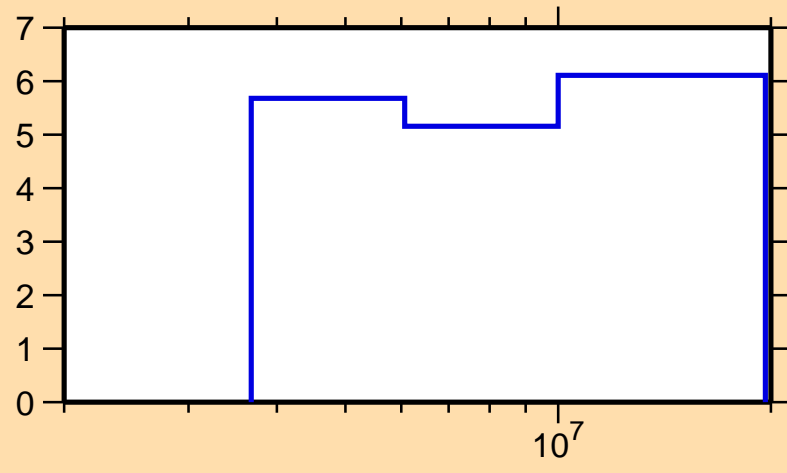
\Delta\sigma/\sigma vs. E for ^{50}\text{Cr}(n,ncont.)
