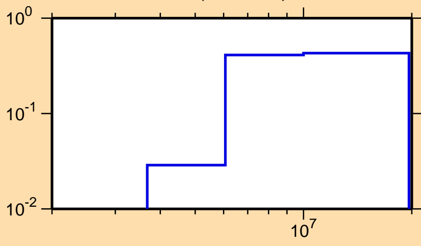
\sigma vs. E for ^{50}\text{Cr}(n,n\text{cont.})
