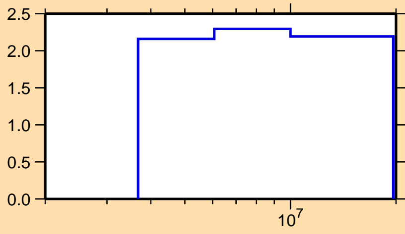
\Delta\sigma/\sigma vs. E for ^{50}\text{Cr}(n,n\text{nonel.})
