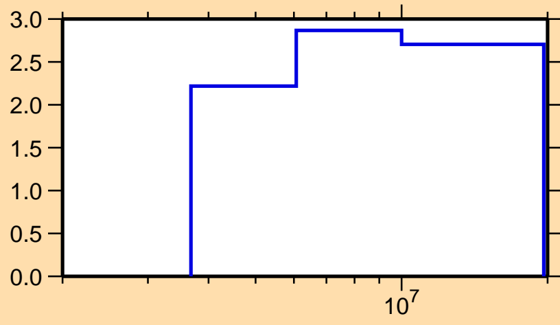
\Delta\sigma/\sigma vs. E for ^{50}\text{Cr}(n,tot.)
