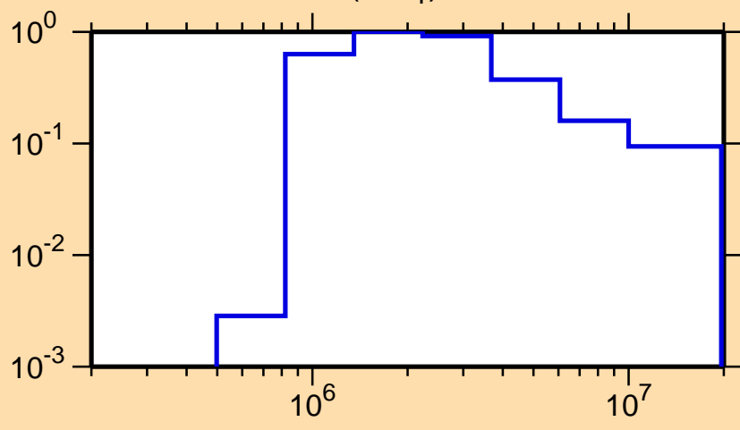
\sigma vs. E for ^{50}\text{Cr}(n,n_1)
