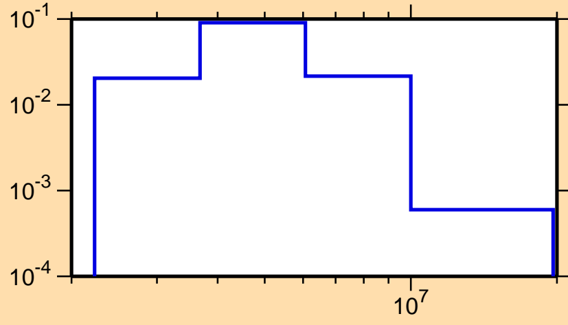
\sigma vs. E for ^{50}\text{Cr}(n,n_4)
