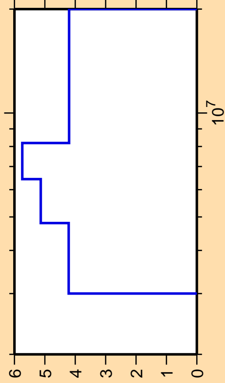
\Delta\sigma/\sigma vs. E for ^{50}\text{Cr}(n,n_4)
