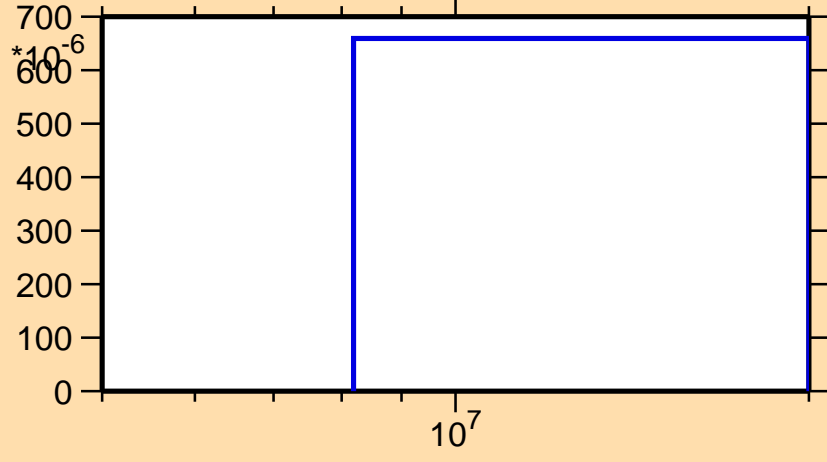
\sigma vs. E for ^{50}\text{Cr}(n,n\alpha)
