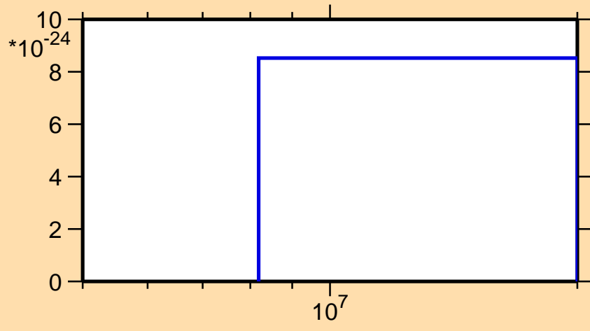
\sigma vs. E for ^{50}\text{Cr}(\text{mt } 45)
