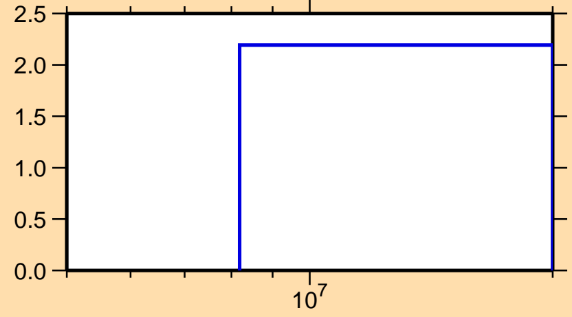
\Delta\sigma/\sigma vs. E for ^{50}\text{Cr}(n,\text{nonel.})
