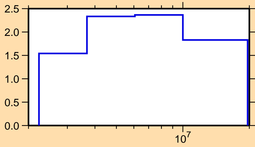
\Delta\sigma/\sigma vs. E for ^{51}\text{Cr}(n,n\text{onel.})
