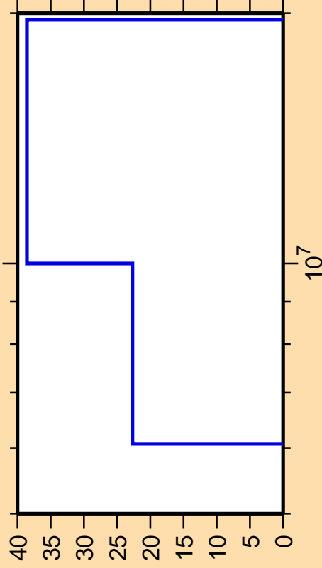
\Delta\sigma/\sigma vs. E for ^{51}\text{Cr}(n,n_1)
