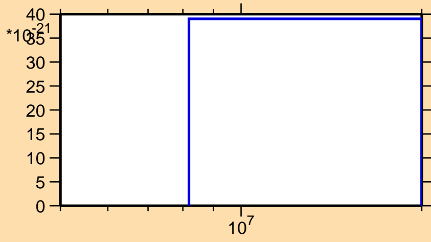
\sigma vs. E for ^{51}\text{Cr}(\text{mt } 34)
