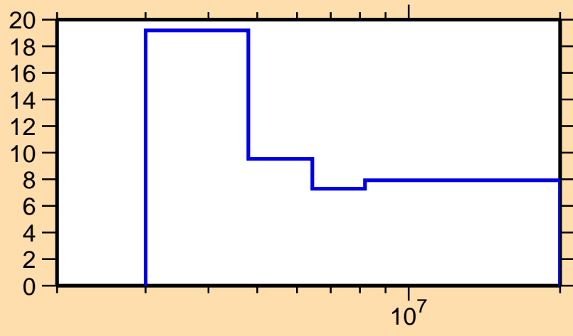
\Delta\sigma/\sigma vs. E for ^{51}\text{Cr}(n,ncont.)
