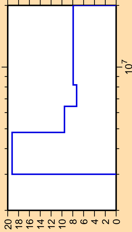
\Delta\sigma/\sigma vs. E for ^{51}\text{Cr}(n,\text{ncont.})
