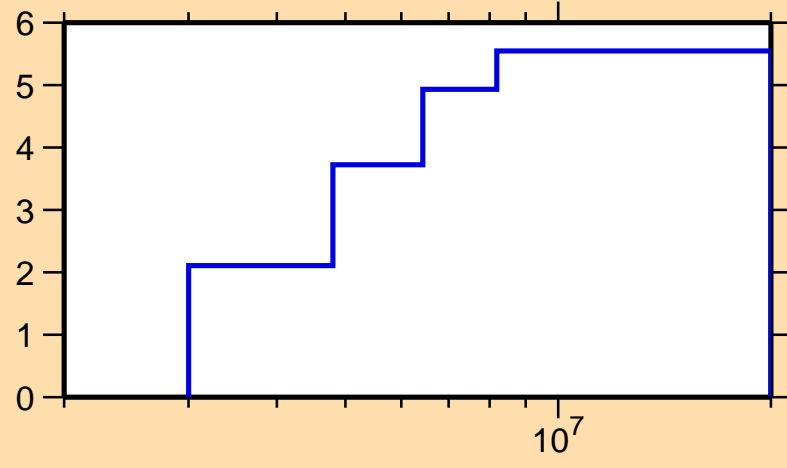
\Delta\sigma/\sigma vs. E for ^{51}\text{Cr}(n,\text{inel.})
