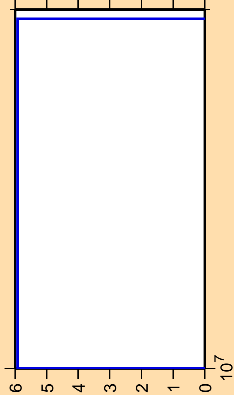
\Delta\sigma/\sigma vs. E for ^{52}\text{Cr}(n,\text{pd})
