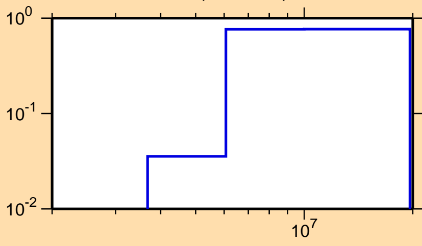
\sigma vs. E for ^{52}\text{Cr}(n,n\text{cont.})
