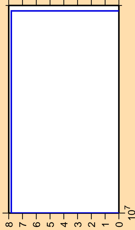
\Delta\sigma/\sigma vs. E for ^{52}\text{Cr}(n,p\alpha)
