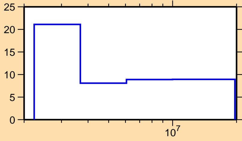
\Delta\sigma/\sigma vs. E for ^{53}\text{Cr}(n,p)
