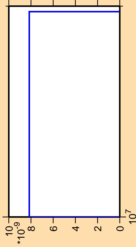
\Delta\sigma/\sigma vs. E for ^{53}\text{Cr} (mt 34)
