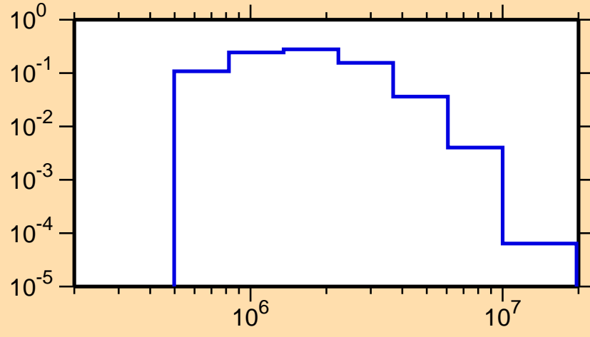
\sigma vs. E for ^{53}\text{Cr}(n,n_1)
