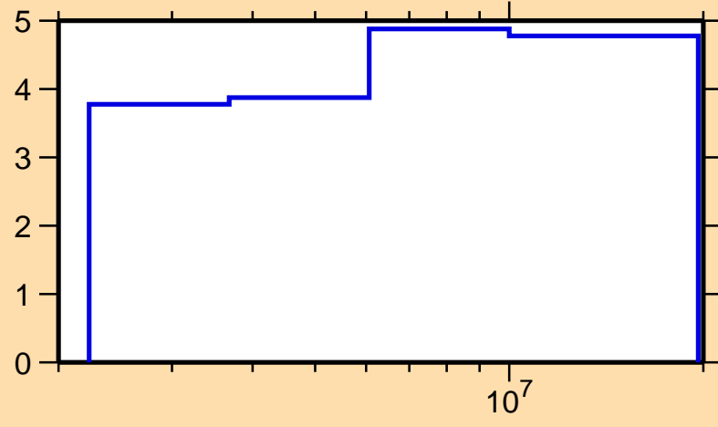
\Delta\sigma/\sigma vs. E for ^{53}\text{Cr}(n,el.)
