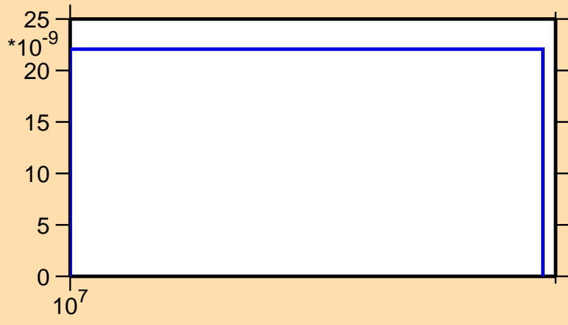
\sigma vs. E for ^{53}\text{Cr}(n,nd)
