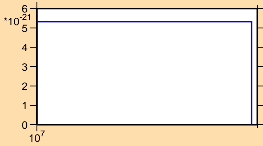
\sigma vs. E for ^{53}\text{Cr} (mt 34)
