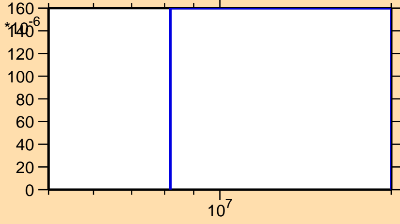
\sigma vs. E for ^{53}\text{Cr}(n,t)
