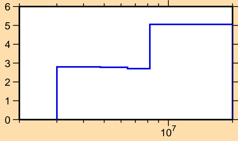
\Delta\sigma/\sigma vs. E for ^{53}\text{Cr}(n,n\text{cont.})
