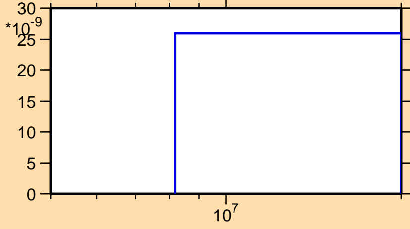
\sigma vs. E for ^{53}\text{Cr}(n,\text{nd})
