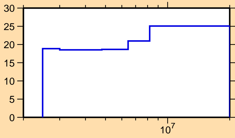
\Delta\sigma/\sigma vs. E for ^{53}\text{Cr}(n,\gamma)
