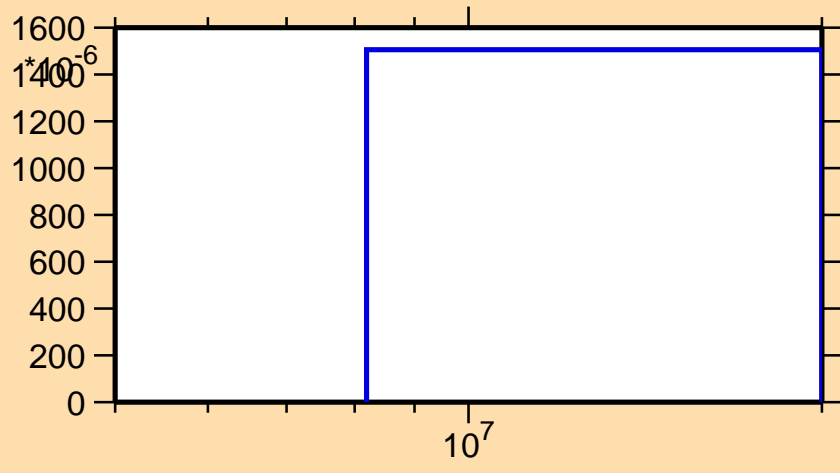
\sigma vs. E for ^{53}\text{Cr}(n,d)
