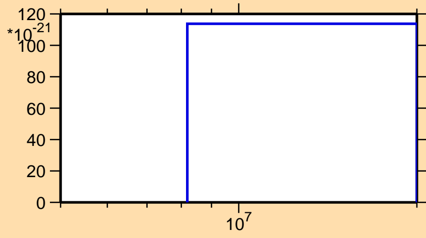
\sigma vs. E for ^{53}\text{Cr}(n,\text{pt})
