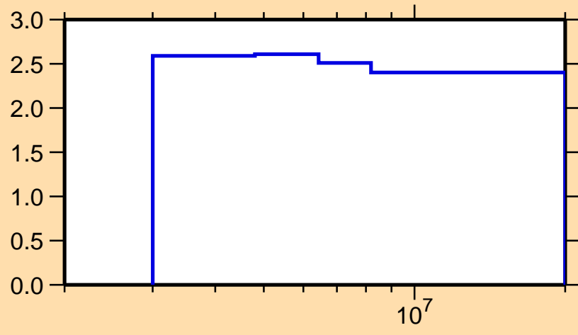
\Delta\sigma/\sigma vs. E for ^{53}\text{Cr}(n,n\text{onel.})
