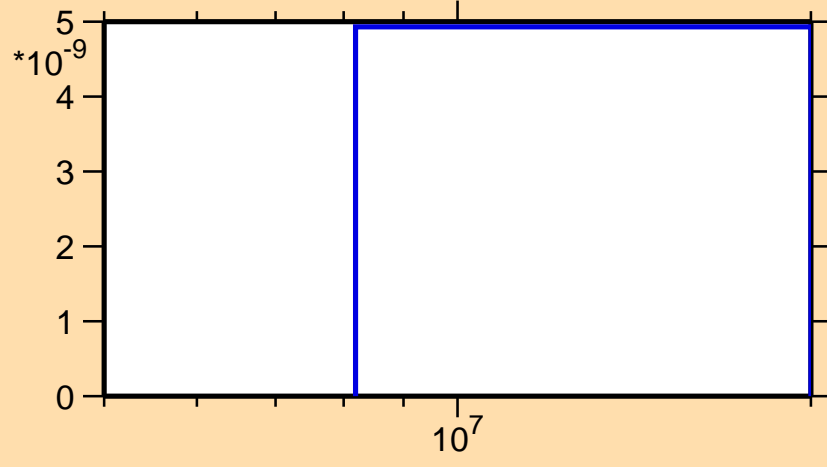
\sigma vs. E for ^{53}\text{Cr}(n,p\alpha)
