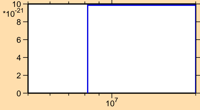
\sigma vs. E for ^{53}\text{Cr}(\text{mt } 34)
