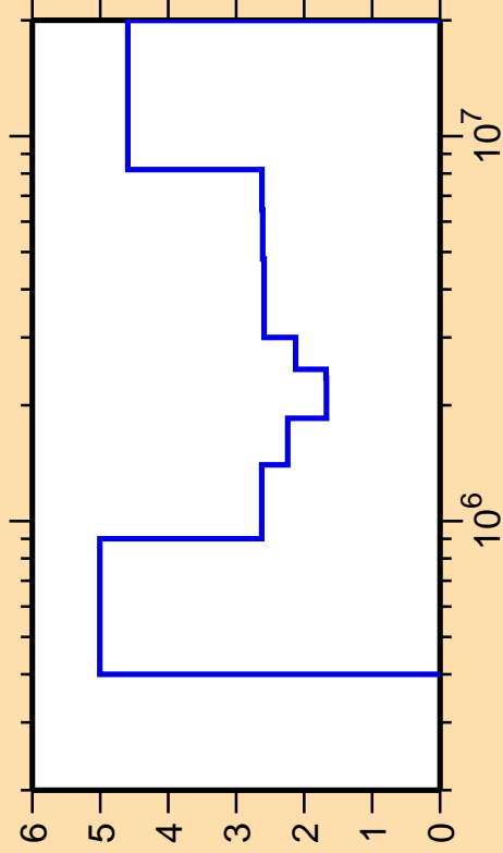
\Delta\sigma/\sigma vs. E for ^{53}\text{Cr}(n,\text{inel.})
