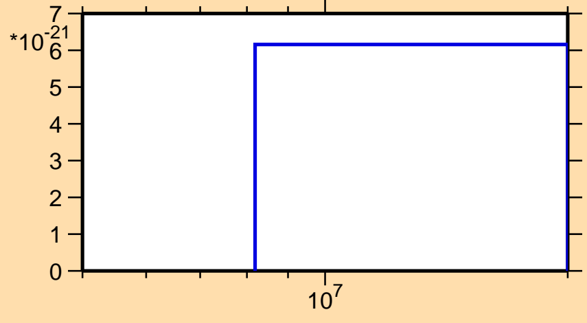
\sigma vs. E for ^{53}\text{Cr}(n,\text{pd})
