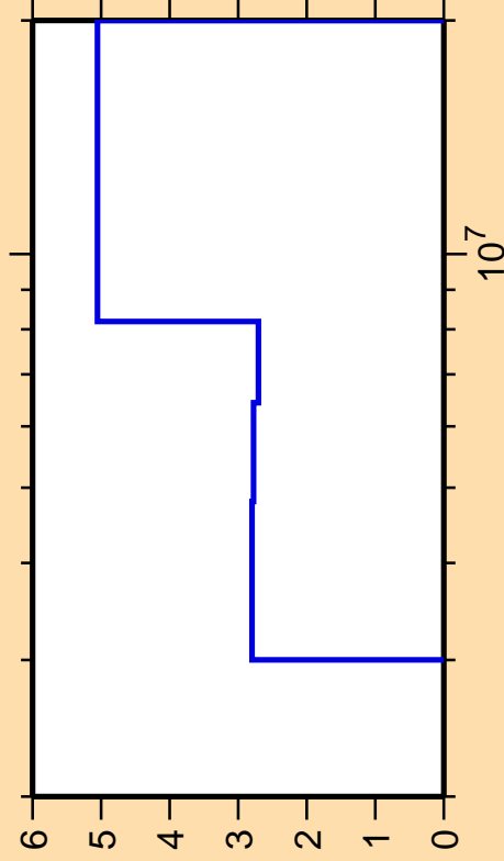
\Delta\sigma/\sigma vs. E for ^{53}\text{Cr}(n,n\text{cont.})
