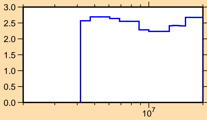
\Delta\sigma/\sigma vs. E for ^{54}\text{Cr}(n,n\text{onel.})
