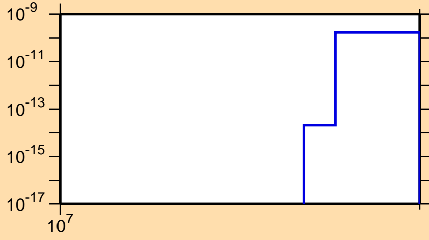
\sigma vs. E for ^{54}\text{Cr}(n,\text{He}3)
