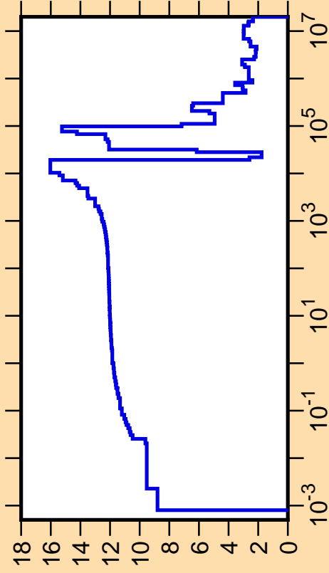
\Delta\sigma/\sigma vs. E for ^{54}\text{Cr}(n,\text{tot.})
