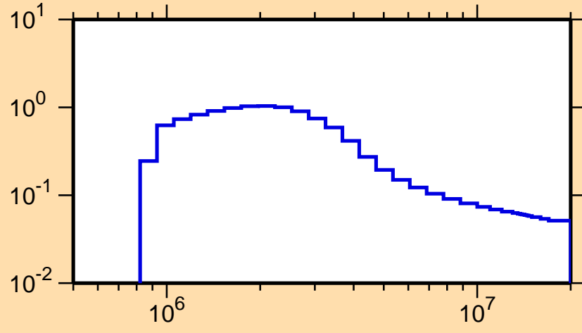
\sigma vs. E for ^{54}\text{Cr}(n,n_1)
