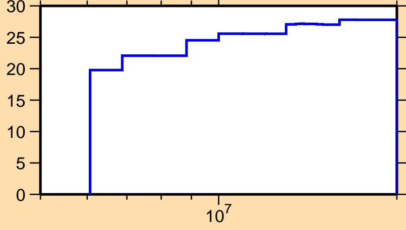
\Delta\sigma/\sigma vs. E for ^{54}\text{Cr}(n,\gamma)
