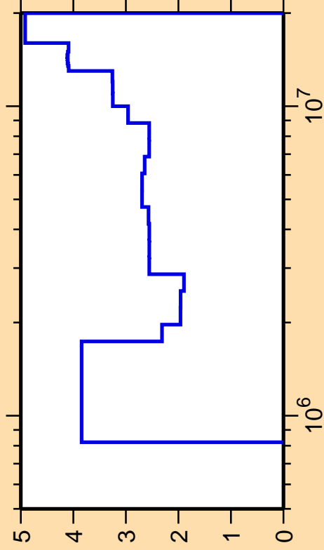
\Delta\sigma/\sigma vs. E for ^{54}\text{Cr}(n,\text{inel.})
