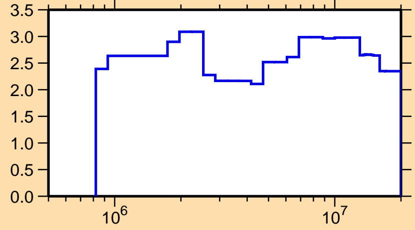
\Delta\sigma/\sigma vs. E for ^{54}\text{Cr}(n,\text{tot.})
