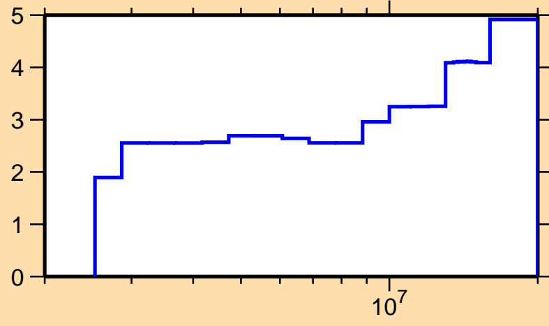
\Delta\sigma/\sigma vs. E for ^{54}\text{Cr}(n,\text{inel.})
