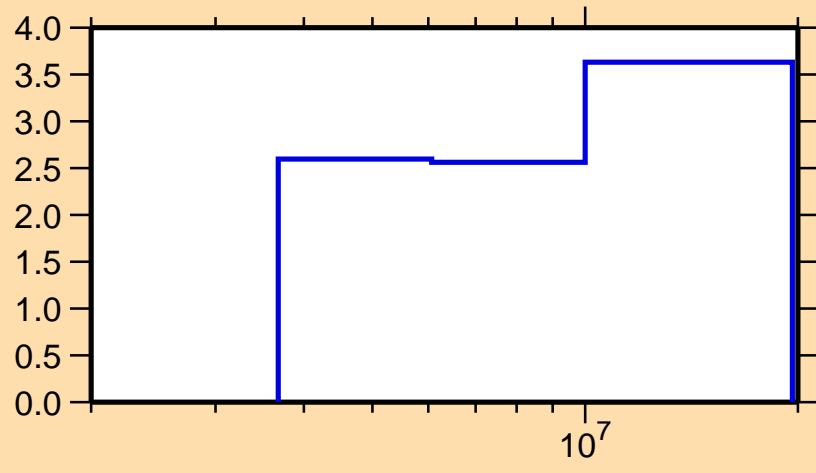
\Delta\sigma/\sigma vs. E for ^{54}\text{Cr}(n,inel.)
