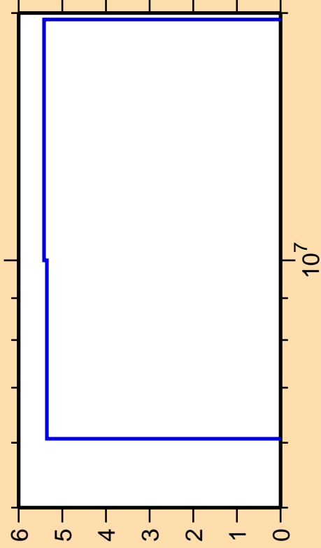
\Delta\sigma/\sigma vs. E for ^{54}\text{Cr}(n,n\text{cont.})
