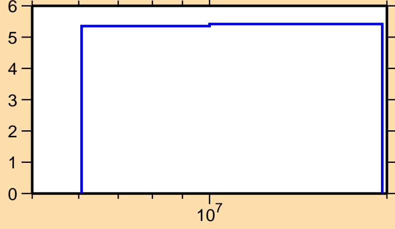
\Delta\sigma/\sigma vs. E for ^{54}\text{Cr}(n,ncont.)
