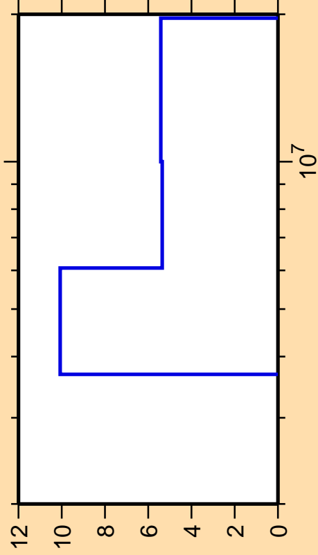
\Delta\sigma/\sigma vs. E for ^{54}\text{Cr}(n,ncont.)
