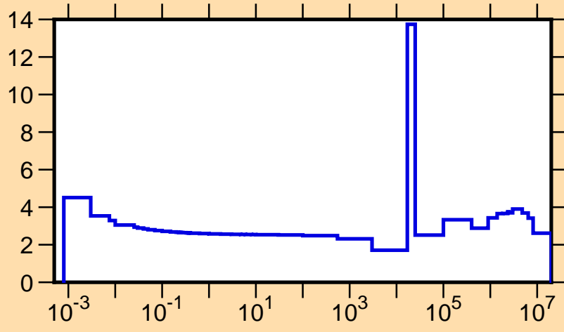
\sigma vs. E for ^{54}\text{Cr}(n,\text{tot.})
