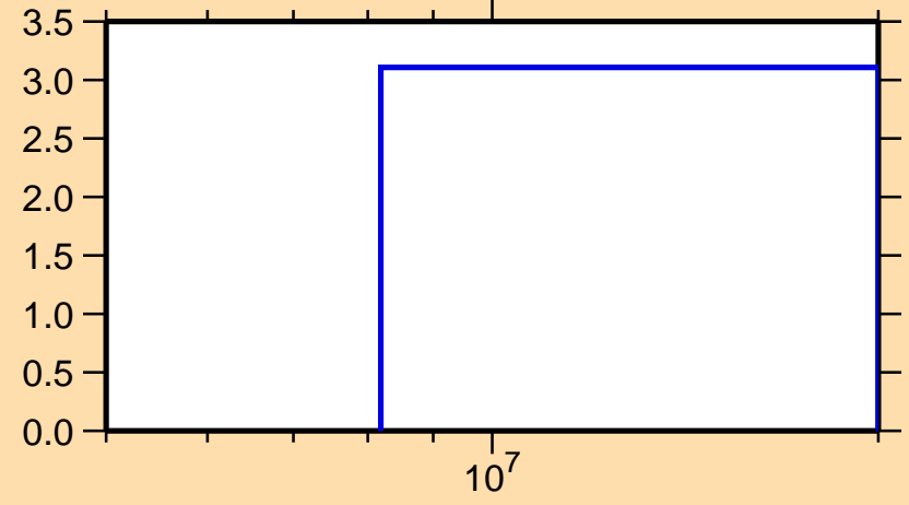
\Delta\sigma/\sigma vs. E for ^{54}\text{Cr}(n,\text{inel.})
