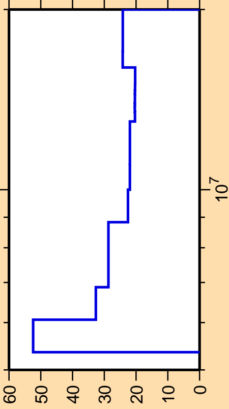
\Delta\sigma/\sigma vs. E for ^{55}\text{Cr}(n,p)
