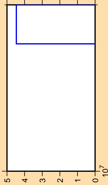
\Delta\sigma/\sigma vs. E for ^{55}\text{Cr}(n,2np)
