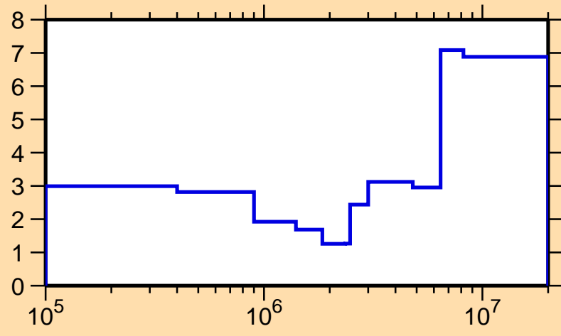
\Delta\sigma/\sigma vs. E for ^{55}\text{Cr}(n,\text{inel.})
