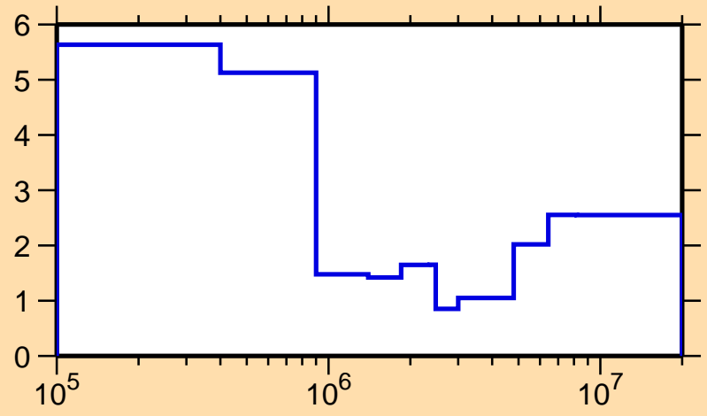
\Delta\sigma/\sigma vs. E for ^{55}\text{Cr}(n,\text{tot.})
