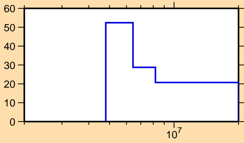
\Delta\sigma/\sigma vs. E for ^{55}\text{Cr}(n,p)
