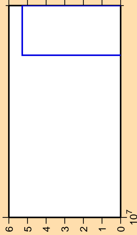
\Delta\sigma/\sigma vs. E for ^{56}\text{Cr}(n,2n\alpha)
