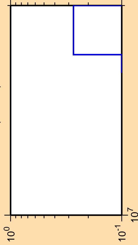
\Delta\sigma/\sigma vs. E for ^{56}\text{Cr}(n,\text{He}3)
