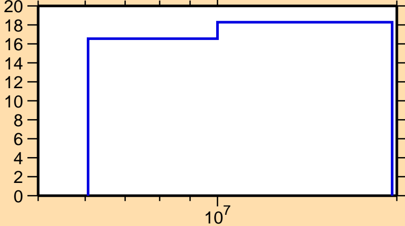
\Delta\sigma/\sigma vs. E for ^{56}\text{Cr}(n,n_1)
