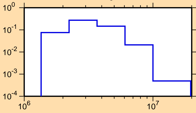
\sigma vs. E for ^{56}\text{Cr}(n,n_3)
