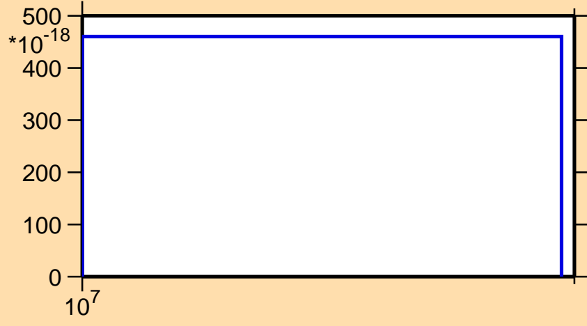
\sigma vs. E for ^{56}\text{Cr}(n,\text{He}3)
