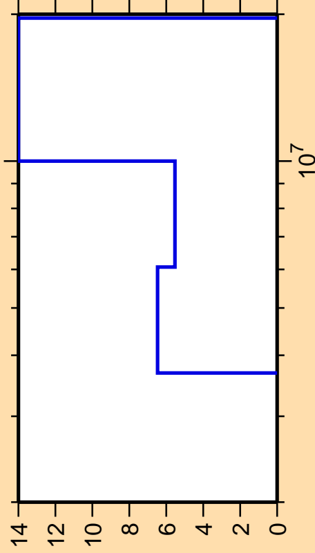
\Delta\sigma/\sigma vs. E for ^{56}\text{Cr}(n,\text{ncont.})
