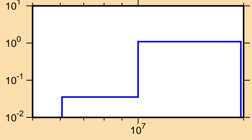
\sigma vs. E for ^{56}\text{Cr}(n,2n)
