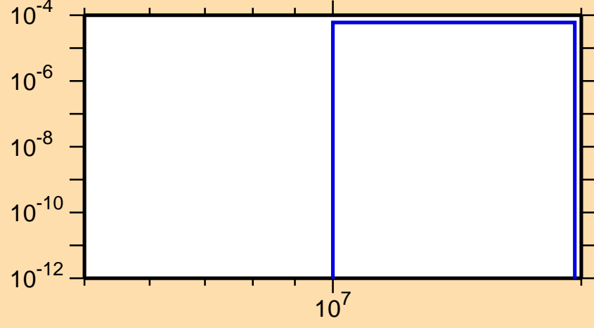
\sigma vs. E for ^{56}\text{Cr}(n,\alpha)
