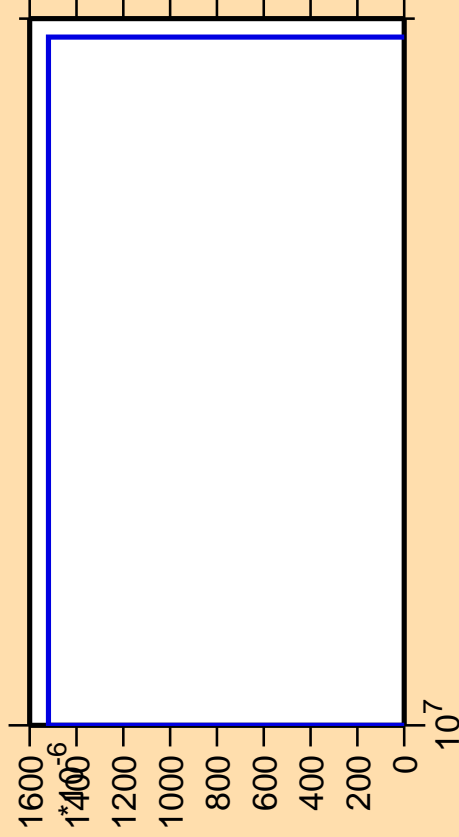
\Delta\sigma/\sigma vs. E for ^{56}\text{Cr}(n,\text{He}3)
