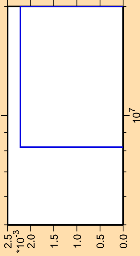
\Delta\sigma/\sigma vs. E for ^{56}\text{Cr}(n,\text{He}3)
