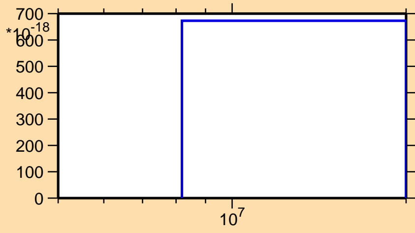
\sigma vs. E for ^{56}\text{Cr}(n,\text{He}3)
