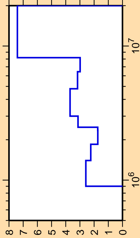
\Delta\sigma/\sigma vs. E for ^{56}\text{Cr}(n,\text{inel.})
