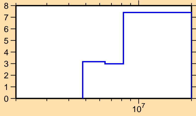
\Delta\sigma/\sigma vs. E for ^{56}\text{Cr}(n,\text{inel.})
