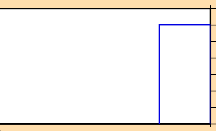
\sigma vs. E for ^{57}\text{Cr}(n,2np)
