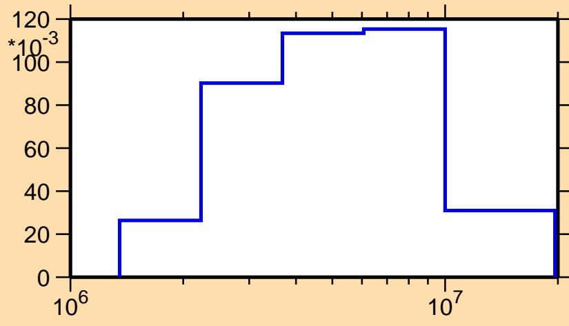
\sigma vs. E for ^{57}\text{Cr}(n,n_4)
