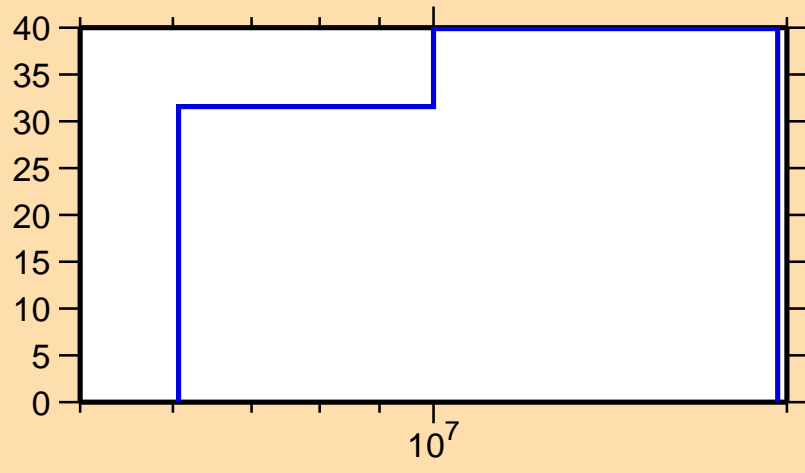
\Delta\sigma/\sigma vs. E for ^{57}\text{Cr}(n,\gamma)
