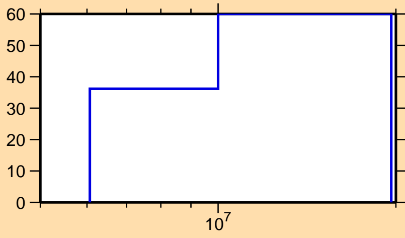
\Delta\sigma/\sigma vs. E for ^{57}\text{Cr}(n,ncont.)
