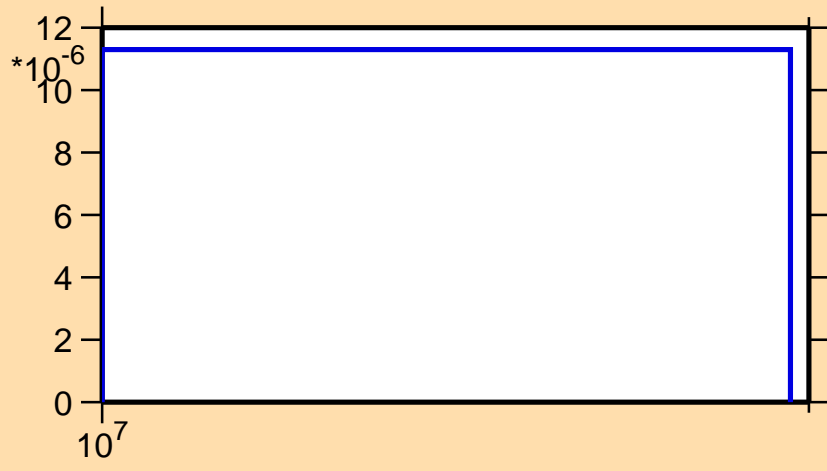
\sigma vs. E for ^{57}\text{Cr}(n,np)
