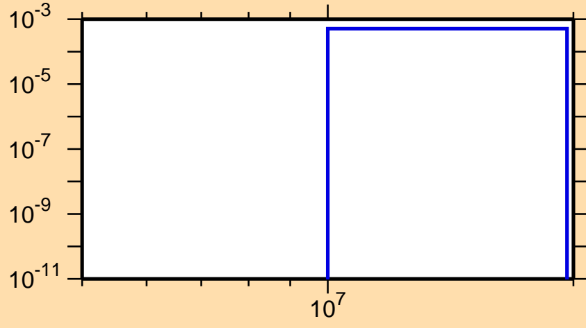
\sigma vs. E for ^{57}\text{Cr}(n,\alpha)
