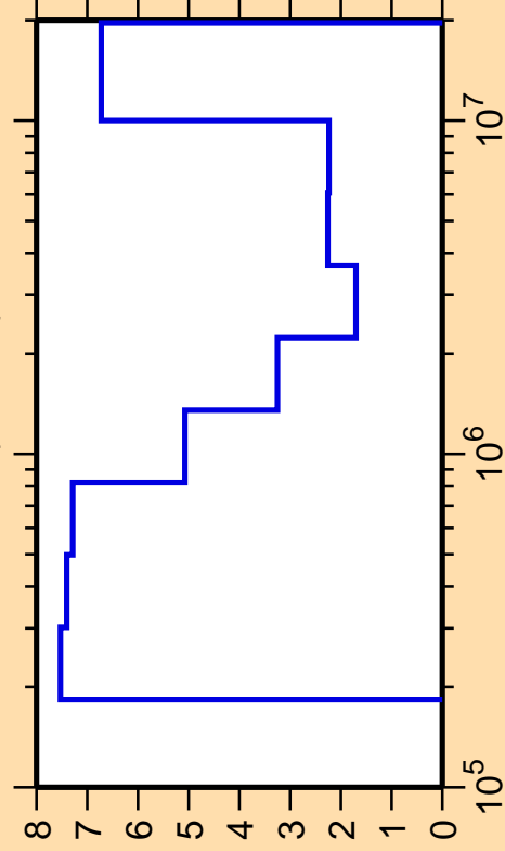
\Delta\sigma/\sigma vs. E for ^{57}\text{Cr}(n,\text{inel.})
