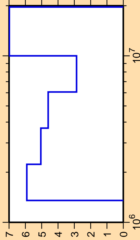
\Delta\sigma/\sigma vs. E for ^{57}\text{Cr}(n,n_4)
