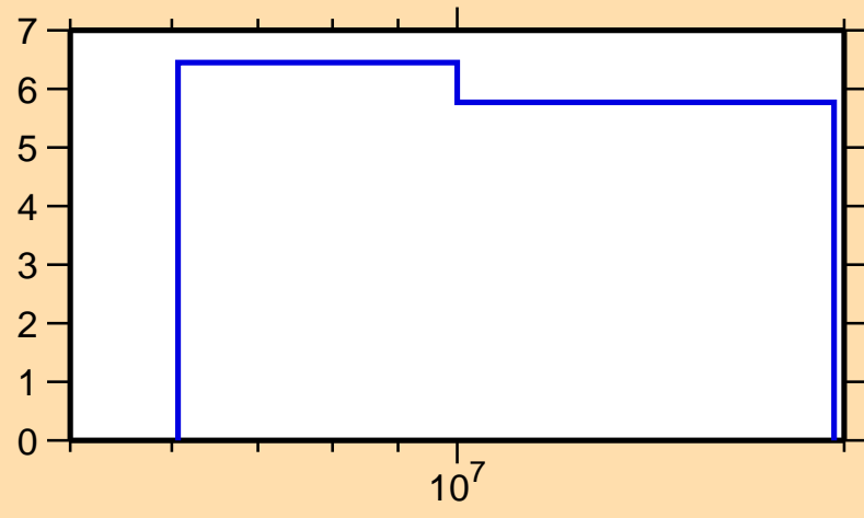
\Delta\sigma/\sigma vs. E for ^{58}\text{Cr}(n,\text{nonel.})
