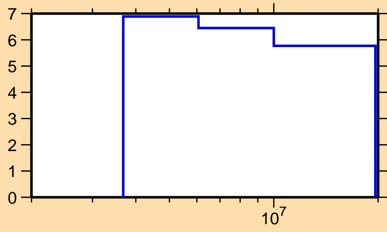
\Delta\sigma/\sigma vs. E for ^{58}\text{Cr}(n,n\text{onel.})
