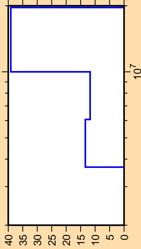
\Delta\sigma/\sigma vs. E for ^{58}\text{Cr}(n,\text{ncont.})
