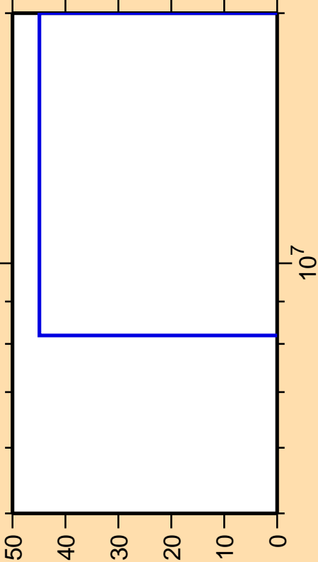
\Delta\sigma/\sigma vs. E for ^{58}\text{Cr}(n,p)
