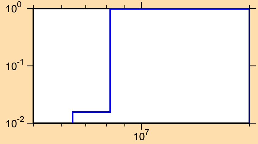
\sigma vs. E for ^{58}\text{Cr}(n,2n)
