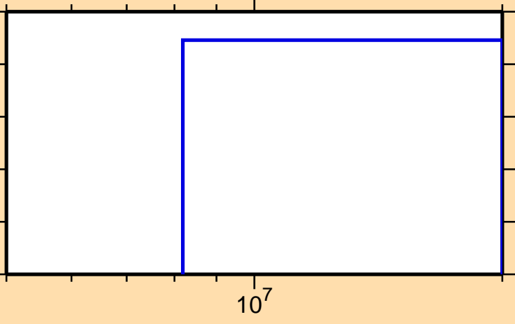
\sigma vs. E for ^{58}\text{Cr}(n,t)
