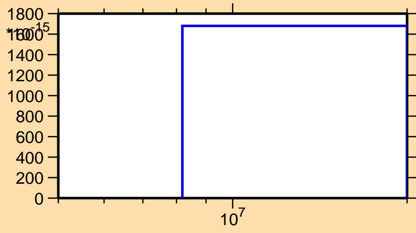
\sigma vs. E for ^{58}\text{Cr}(n,nt)
