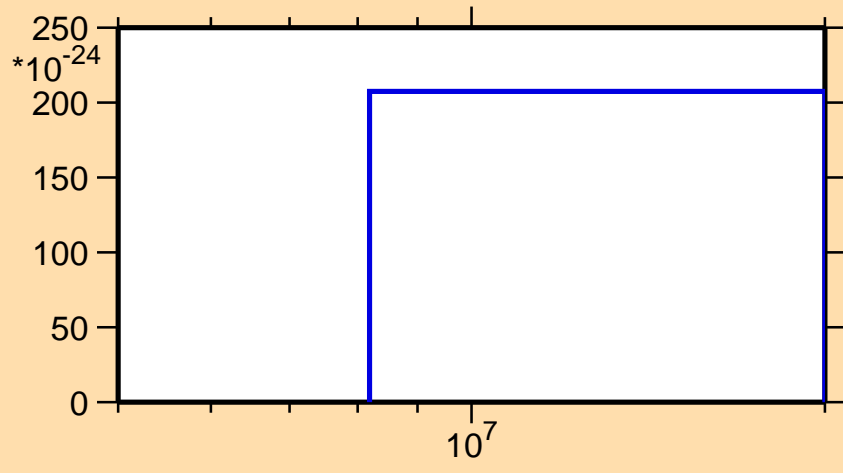
\sigma vs. E for ^{58}\text{Cr}(n,\text{He}3)
