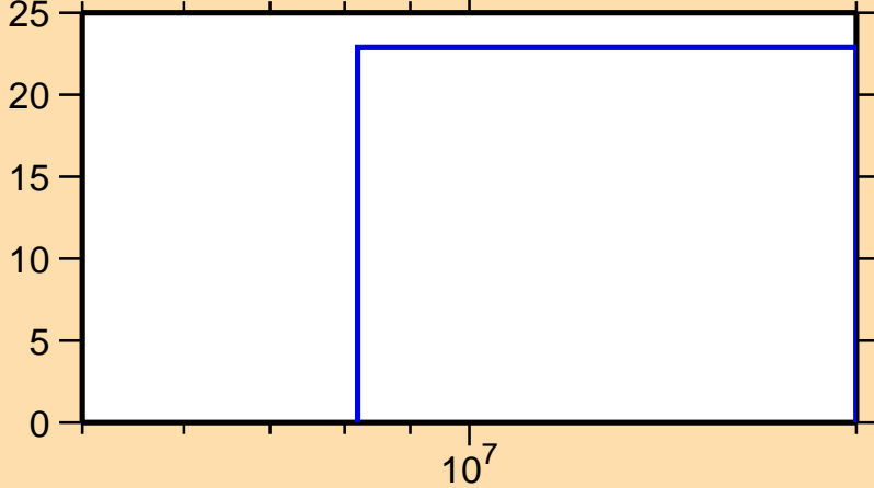
\Delta\sigma/\sigma vs. E for ^{58}\text{Cr}(n,ncont.)
