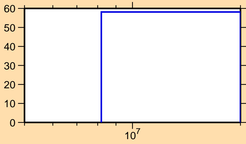
\Delta\sigma/\sigma vs. E for ^{59}\text{Cr}(n,\gamma)
