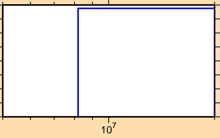
\sigma vs. E for ^{59}\text{Cr}(n,t)
