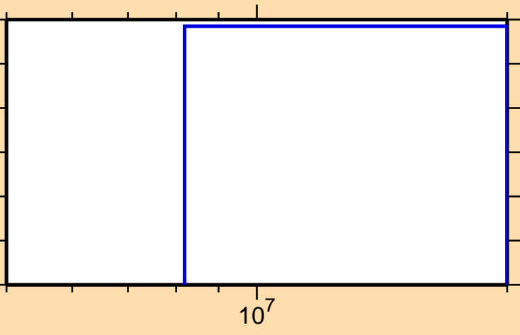
\sigma vs. E for ^{59}\text{Cr}(n,\alpha)
