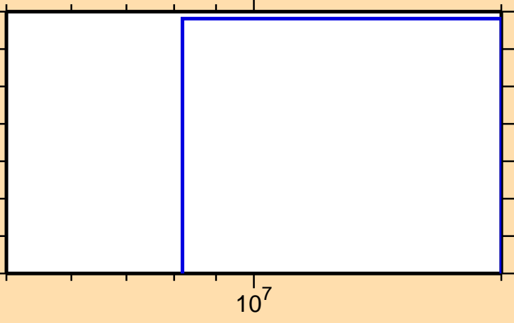
\sigma vs. E for ^{59}\text{Cr}(n,2np)
