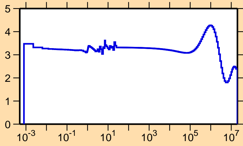
\sigma vs. E for ^{115}\text{Cs}(n,\text{el.})
