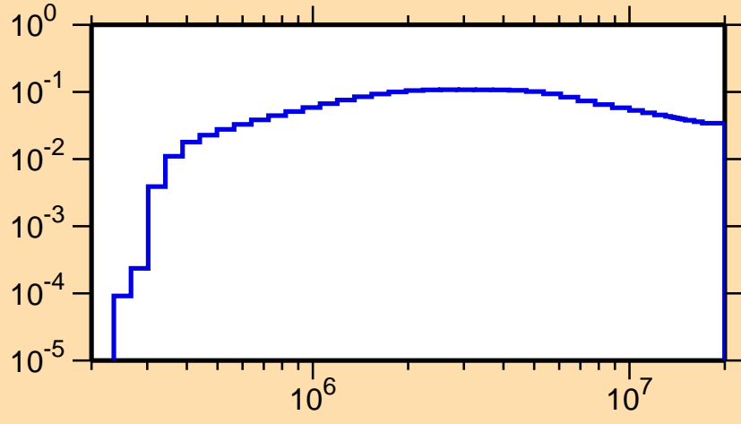
\sigma vs. E for ^{115}\text{Cs}(n,n_1)
