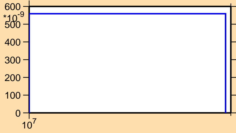
\sigma vs. E for ^{115}\text{Cs}(n,2np)
