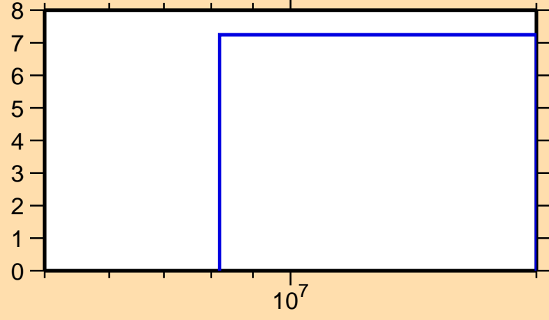
\Delta\sigma/\sigma vs. E for ^{115}\text{Cs}(n,\text{nonel.})
