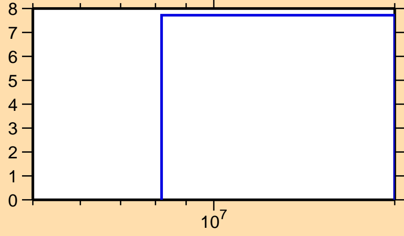
\Delta\sigma/\sigma vs. E for ^{115}\text{Cs}(n,\text{el.})
