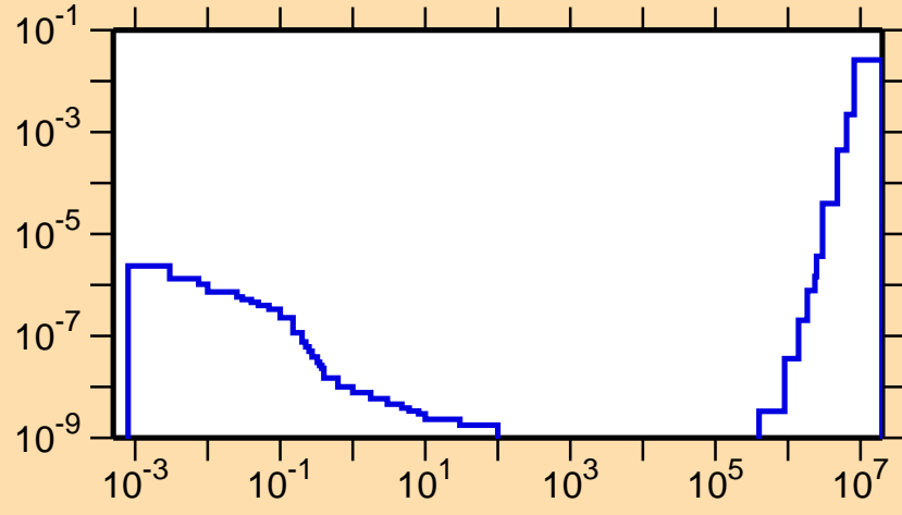
\sigma vs. E for ^{115}\text{Cs}(n,d)
