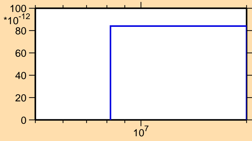
\sigma vs. E for ^{115}\text{Cs}(\text{mt } 34)
