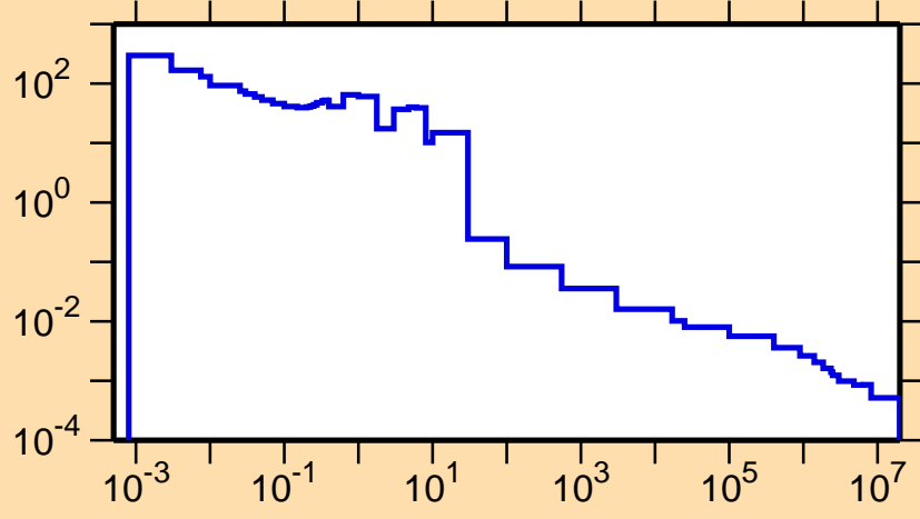
\sigma vs. E for ^{115}\text{Cs}(n,\gamma)
