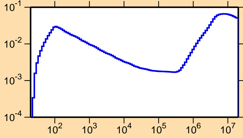
\sigma vs. E for ^{116}\text{Cs}(n,\text{inel.})
