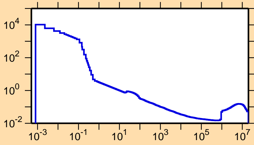
\sigma vs. E for ^{116}\text{Cs}(n,\alpha)
