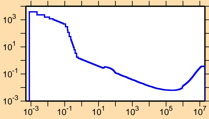
\sigma vs. E for ^{116}\text{Cs}(n,p\alpha)
