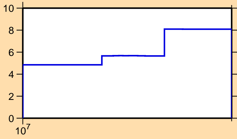
\Delta\sigma/\sigma vs. E for ^{116}\text{Cs}(n,\text{tot.})
