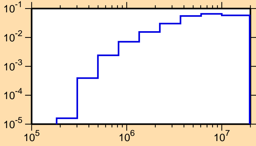
\sigma vs. E for ^{116}\text{Cs}(n,n\text{cont.})
