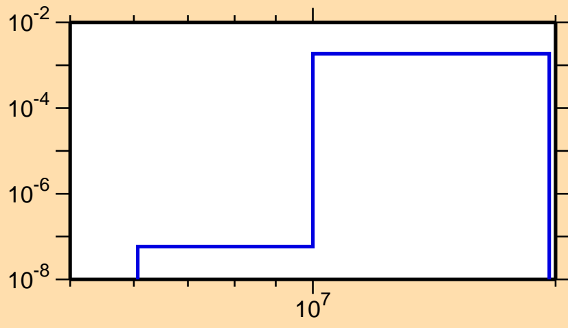
\sigma vs. E for ^{116}\text{Cs}(n,\text{pd})
