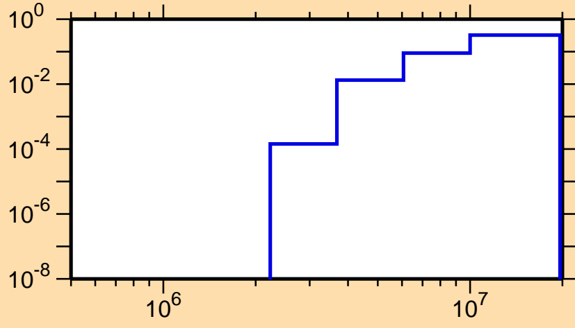
\sigma vs. E for ^{116}\text{Cs}(n,np)
