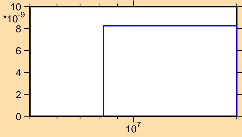
\sigma vs. E for ^{116}\text{Cs}(\text{mt } 34)
